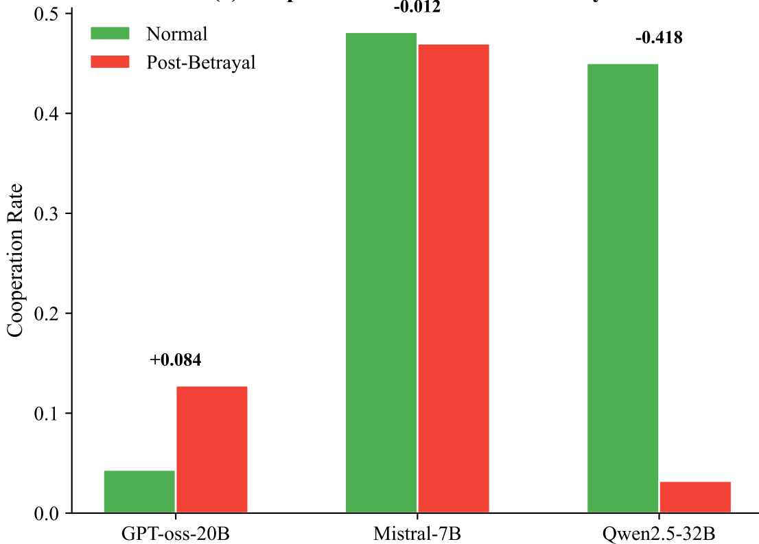
(a) Coop. Rate: Normal vs Post-Betrayal
