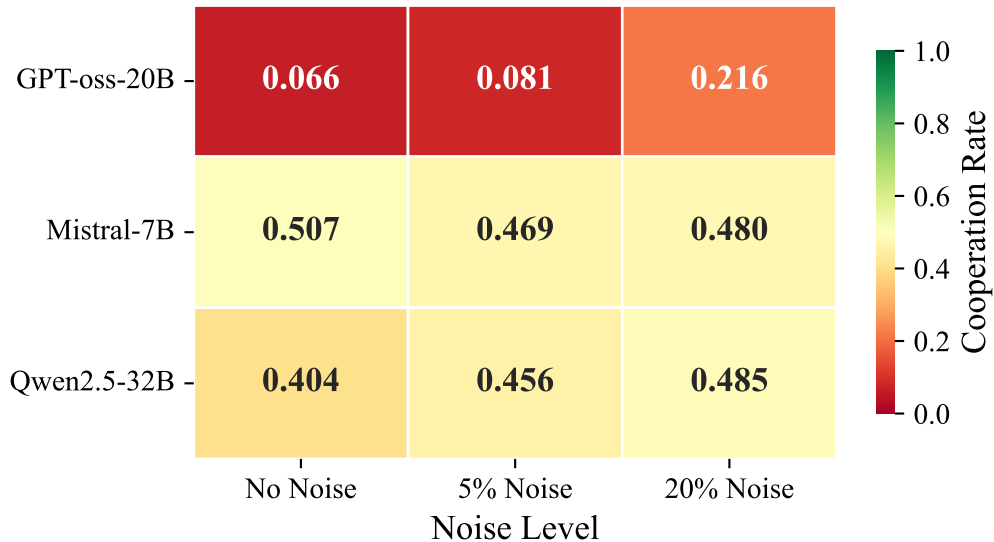
Mean Cooperation Rate by Model and Noise Level
