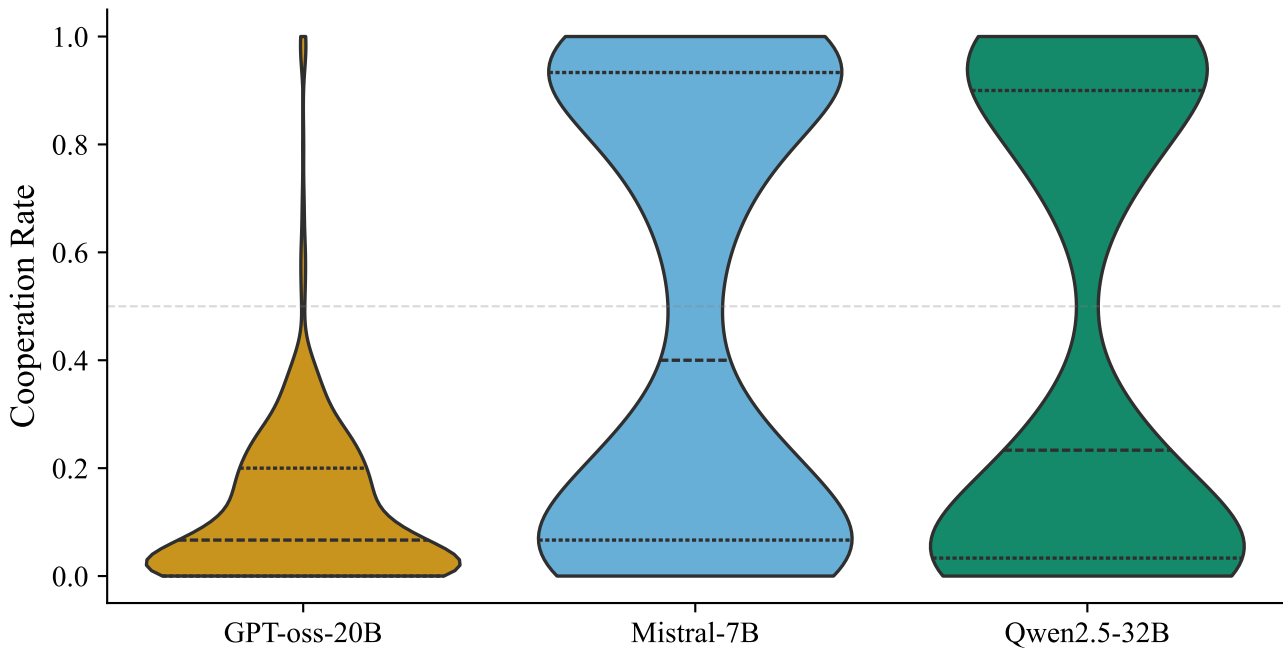
Distribution of Cooperation Rates by Model
