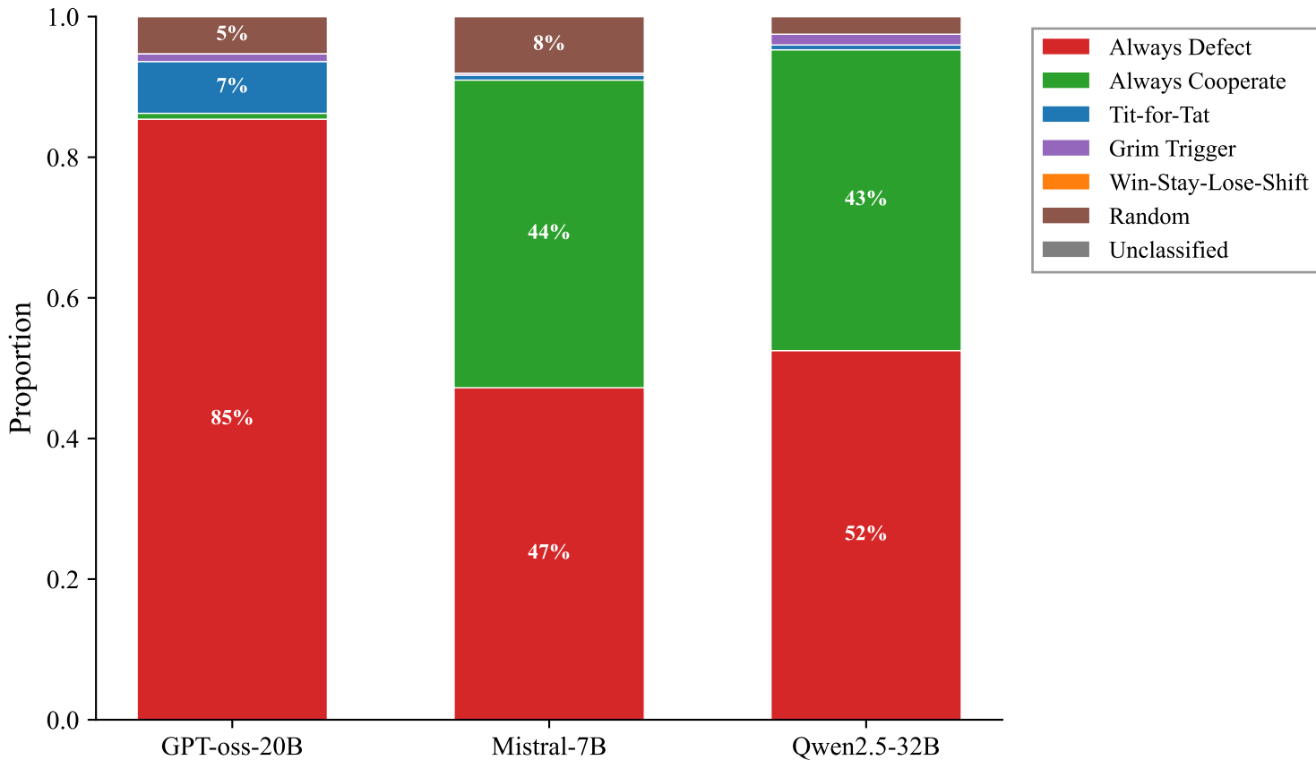
Strategy Classification Distribution by Model
