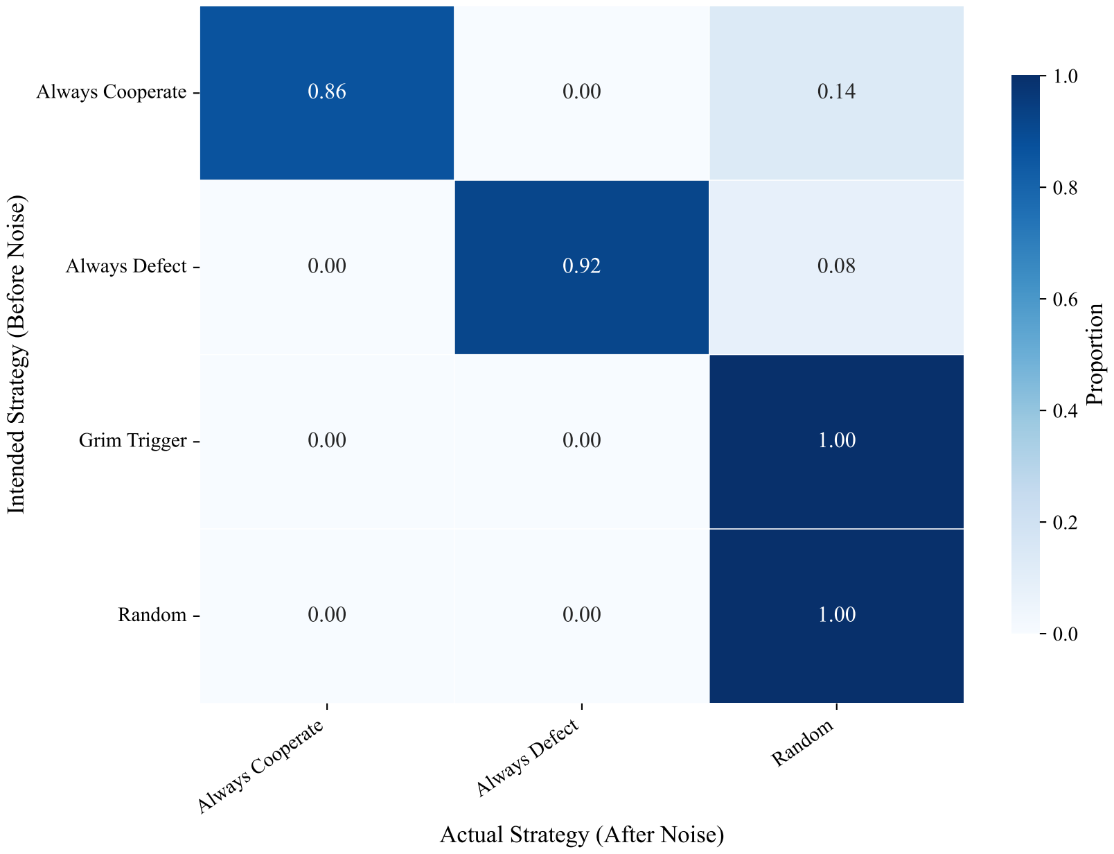
Strategy Confusion Matrix Under 20% Noise
