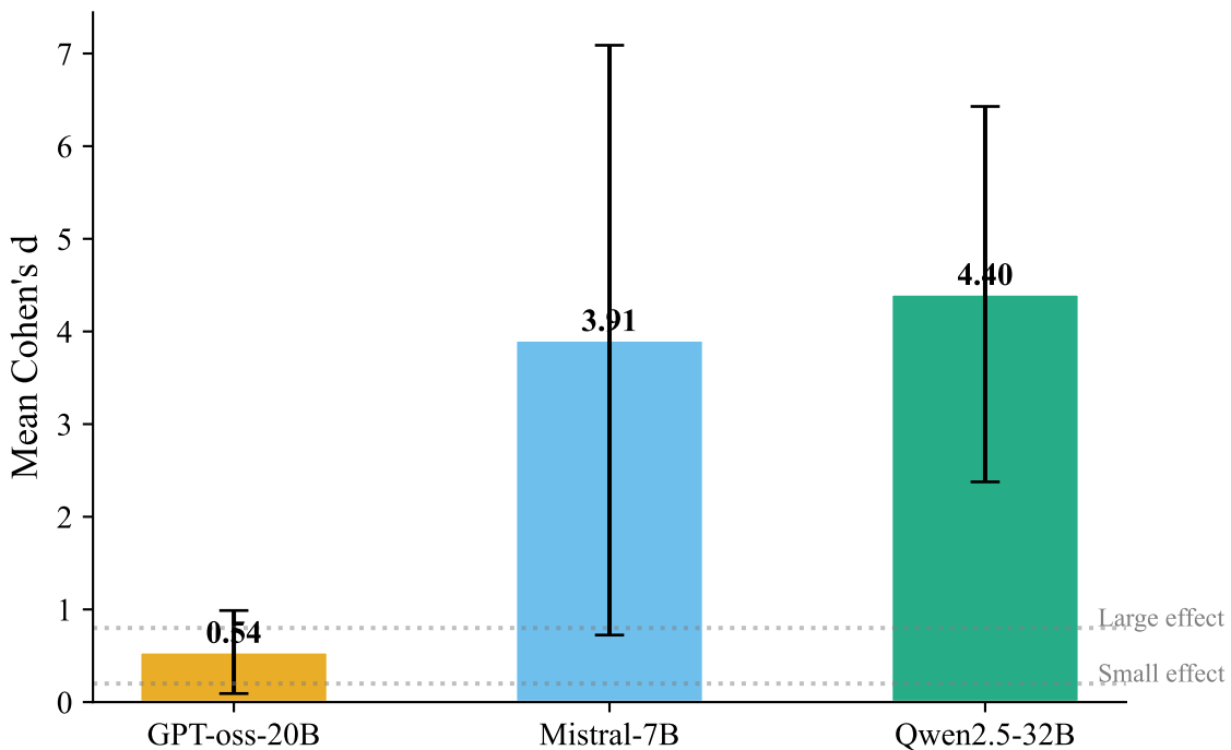
Average Personality Compliance
