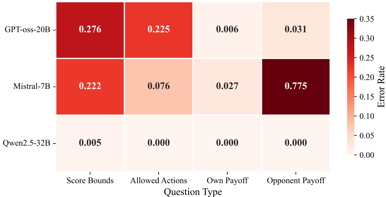
Error Rate by Question Type × Model
