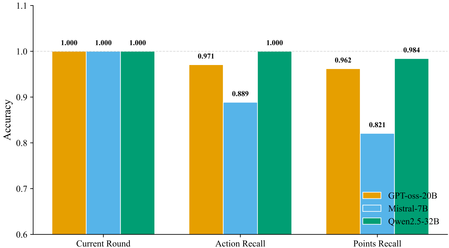
Temporal Awareness by Memory Type
