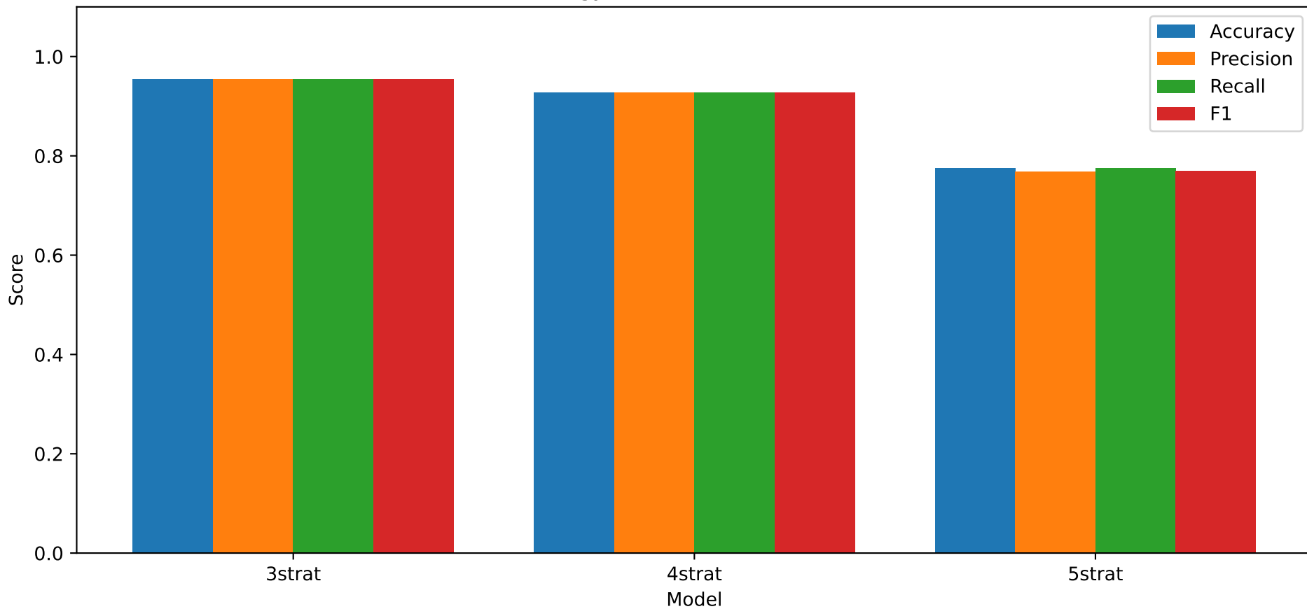
LSTM Strategy Detection Model Performance
