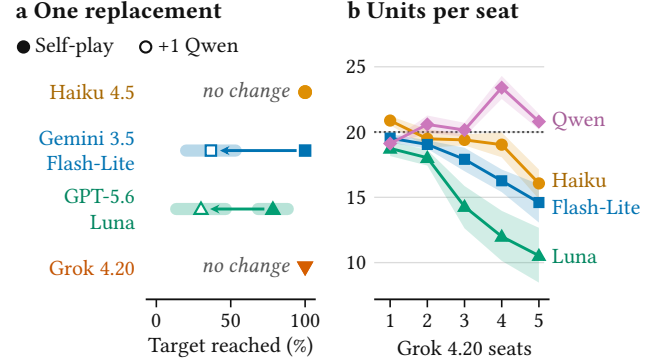
Figure 5: Mixed groups, pooled over p = 0.1, 0.5, 0.9 . (a) Self-play (filled; 60 games, grid plus question games) versus one Qwen3-235B replacement (open; 30); arrows run from the first to the second. (b) Mean contribution per focal seat beside one to five Grok 4.20 seats (30 games each); dotted: fair share. Bars and bands: 95% game-bootstrap intervals, not stratified by risk. Lines join measured means.
