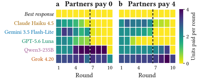
Figure 4: One model beside five scripted partners, pooled over five risk levels (50 games per row). A cell is the mean payment in one round; the top row is the best response, 0 in every round. The dashed rule follows round 6, after which the outcome is settled in most games.
