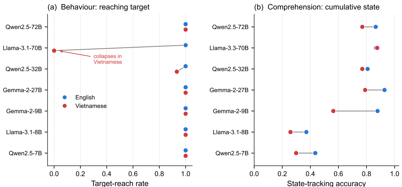
Figure 11. English versus Vietnamese. (a) Target-reach rate in each language for the seven open-weight models, the two points of a pair offset vertically so that coincident values stay visible. Behaviour is identical across languages for five of the seven; Qwen2.5-32B dips slightly (100% to 93.3%) and Llama-3.1-70B collapses from 100% to 0% in Vietnamese. (b) Cumulative-state accuracy in each language. Vietnamese selectively degrades the arithmetic; the largest loss is Gemma-2-9B (31.5 points), while the weakest adders have least left to lose and Llama-3.3-70B is unaffected.
