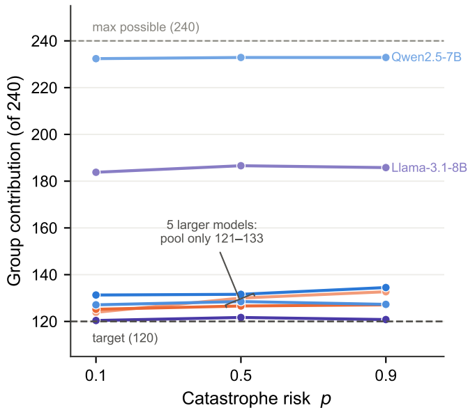
(b) How much they pool
