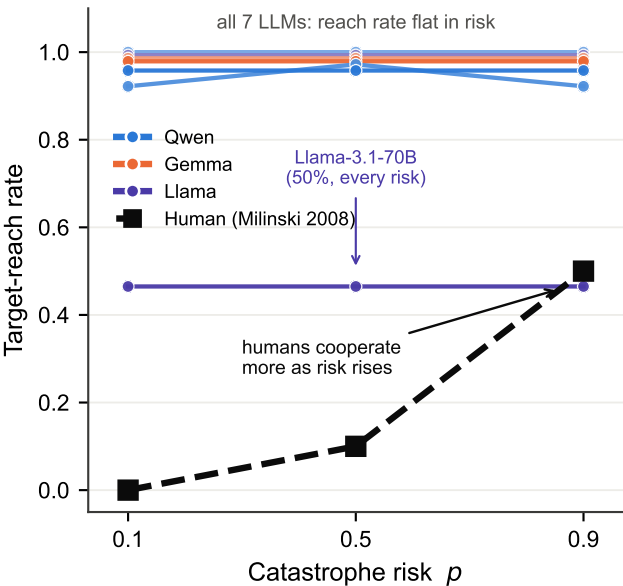
(a) Reaching the collective target
