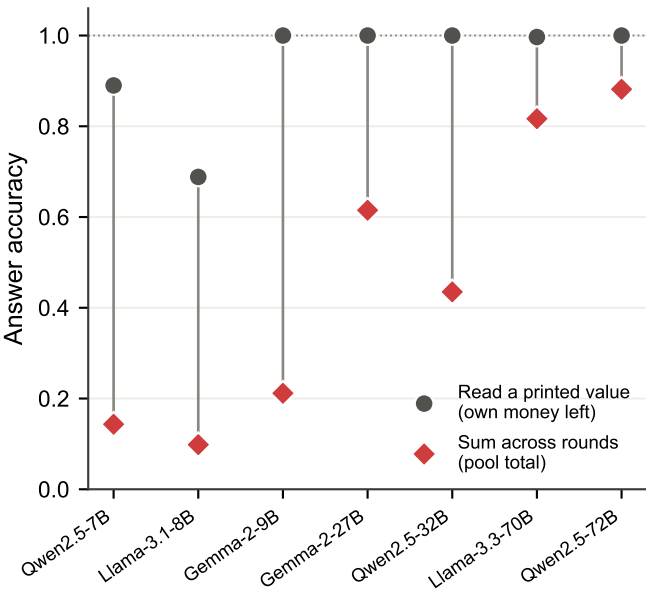
(a) Reading \neq adding
