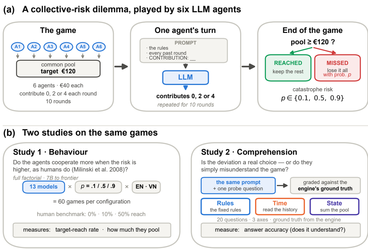
Figure 1. Study design. (a) Six LLM agents play a faithful replication of the Milinski collective-risk dilemma: each of six agents starts with €40 and, over ten rounds, privately contributes 0, 2 or 4 to a common pool from a prompt containing the rules and the full history; at the end, if the pool has not reached €120 the group suffers a catastrophe with probability p \in \{0.1, 0.5, 0.9\} . (b) The same games feed two studies. Study 1 (behaviour) crosses the model panel with three risk levels and two languages and measures the target-reach rate and how much the agents pool. Study 2 (comprehension) appends a graded question to the identical prompt, scoring twenty questions along three axes (Rules, Time, State) against the engine's ground truth, to ask whether any deviation is a genuine choice or a misunderstanding.
