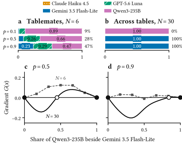
Figure 6: Which model selection favours ( \alpha -Rank, \beta = 1 ). (a, b) Stationary mass of each model when agents are compared with tablemates ( N = 6 ) or mostly with agents at other tables ( N = 30 ); right of each bar, the self-play target rate weighted by mass. (c, d) Gradient of selection, the expected change in the share of Qwen3-235B in a population with Gemini 3.5 Flash-Lite; black circles are fixed points, filled if stable and open if unstable; grey squares are the states of a population of six. Invasion diagrams for all pairs are in the supplementary material.
