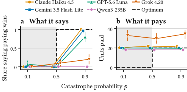
Figure 3: What the questioned seat says and does in the same games (ten per model and risk level), with 95% intervals. (a) Share of value-question answers saying that paying every round gives the higher average cash; dashed: the correct answer. (b) Units the seat pays; dashed: the optimum of Proposition 1.
