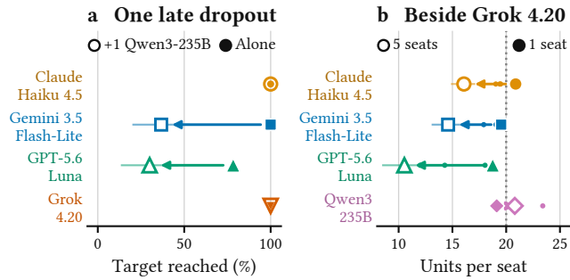
Figure 5: Two models at one table, pooled over p . Arrows run from the filled marker to the open one, which carries a 95% interval. (a) Target reached by six seats of one model (60 games) and by five seats plus one Qwen3-235B seat (30). (b) What a seat pays beside one and five Grok 4.20 seats (30 games each; dots: two to four); dotted: the fair share.
