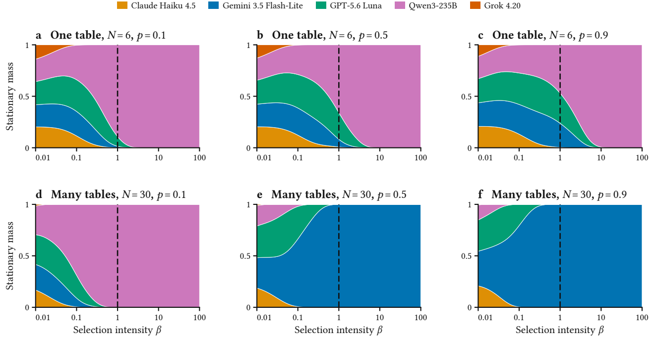
Figure S5: Stationary mass of the five models as the selection intensity \beta grows from 0.01 to 100. Top: a population of one table ( N = 6 ). Bottom: a larger population ( N = 30 ). The dashed line marks \beta = 1 , the setting of Figure 6 of the paper.
