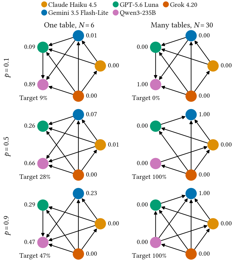
Figure S6: Invasion diagrams (rare-mutation Fermi selection, \beta = 1 ), computed and drawn with EGTtools. A node is a one-model population, with its stationary mass beside it. An arrow from A to B means that one B newcomer takes over an A population with more than the neutral probability 1/N . Left: one table, N = 6 . Right: larger randomly mixed population, N = 30 . Bottom left: self-play target rate weighted by mass.
