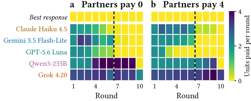
Figure S3: One model beside five scripted partners, pooled over five risk levels (50 games per row). A cell is the mean payment in one round; the top row is the best response, 0 in every round. The dashed rule follows round 6, after which the outcome is settled in most games.
