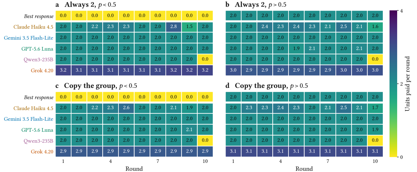
Figure S4: Mean payment in each round beside partners who always pay 2 (top) and partners who copy the group (bottom), at low risk ( p = 0.1 and 0.3 , left) and high risk ( p = 0.7 and 0.9 , right); 20 games per row. The top row of each panel is the best response. Above p^* any sequence that adds up to 20 is a best response, and the row shows their round-by-round average, which is 2.
