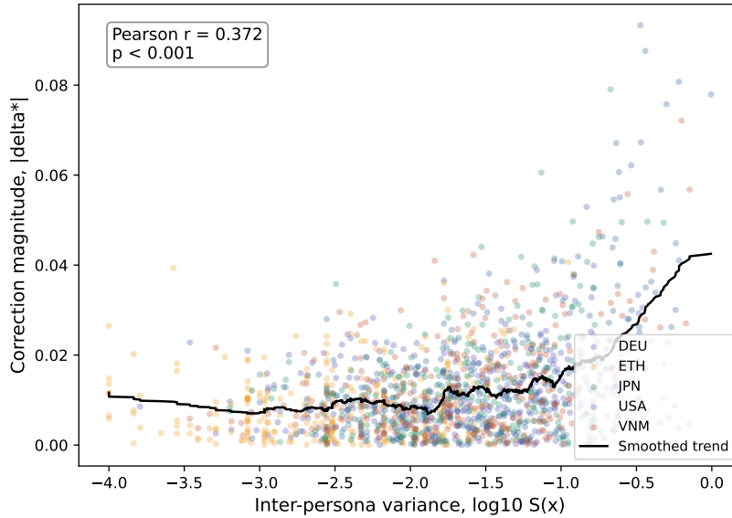
Figure 5: Scenario-level conditioning of the DISCA correction. Per-scenario inter-persona variance (log scale) versus DISCA correction magnitude |\delta^*| , n = 1,550 scenarios across five countries on Qwen2.5-7B. Each dot is one scenario; the black curve is a Savitzky–Golay smoothed trend. Pearson r = +0.372 , p < 10^{-3} : when personas agree (left), DISCA applies near-zero corrections; when they disagree (right), DISCA applies larger corrections. The trend is positive but bounded, so high-disagreement scenarios do not lead to runaway correction magnitudes; isolating how much of this saturation is contributed by the dual-pass reliability gate (versus the IS proposal scale) would require a no-gate ablation that we leave to future work.
