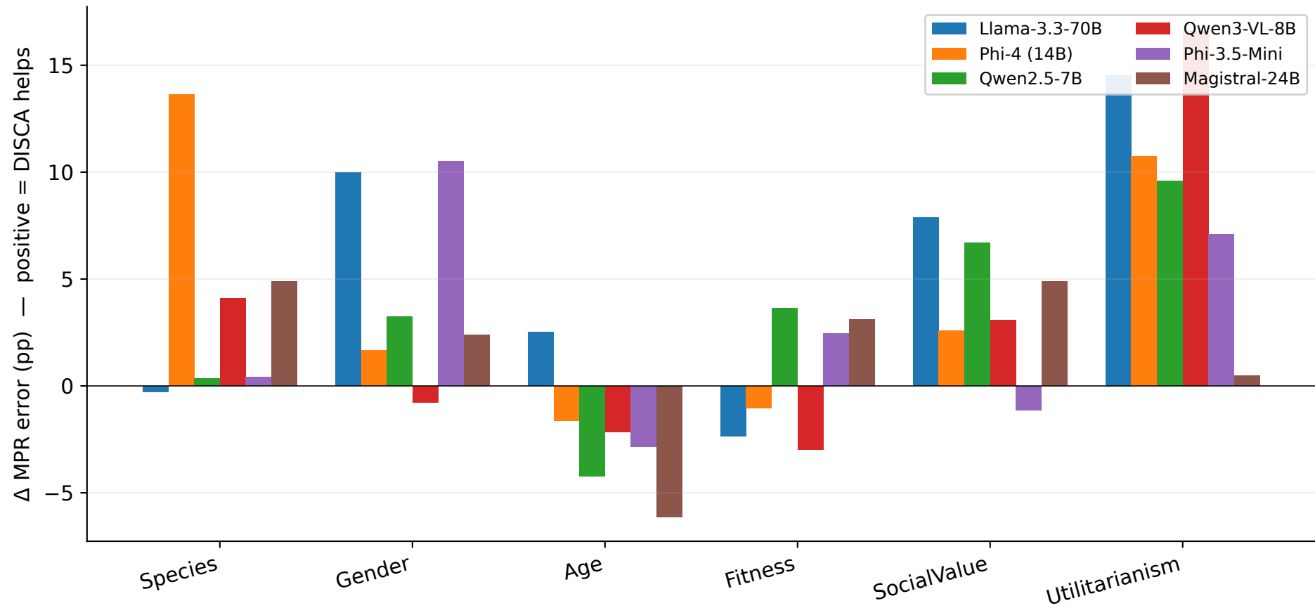
Per-dimension DISCA gain on the headline 6 models
