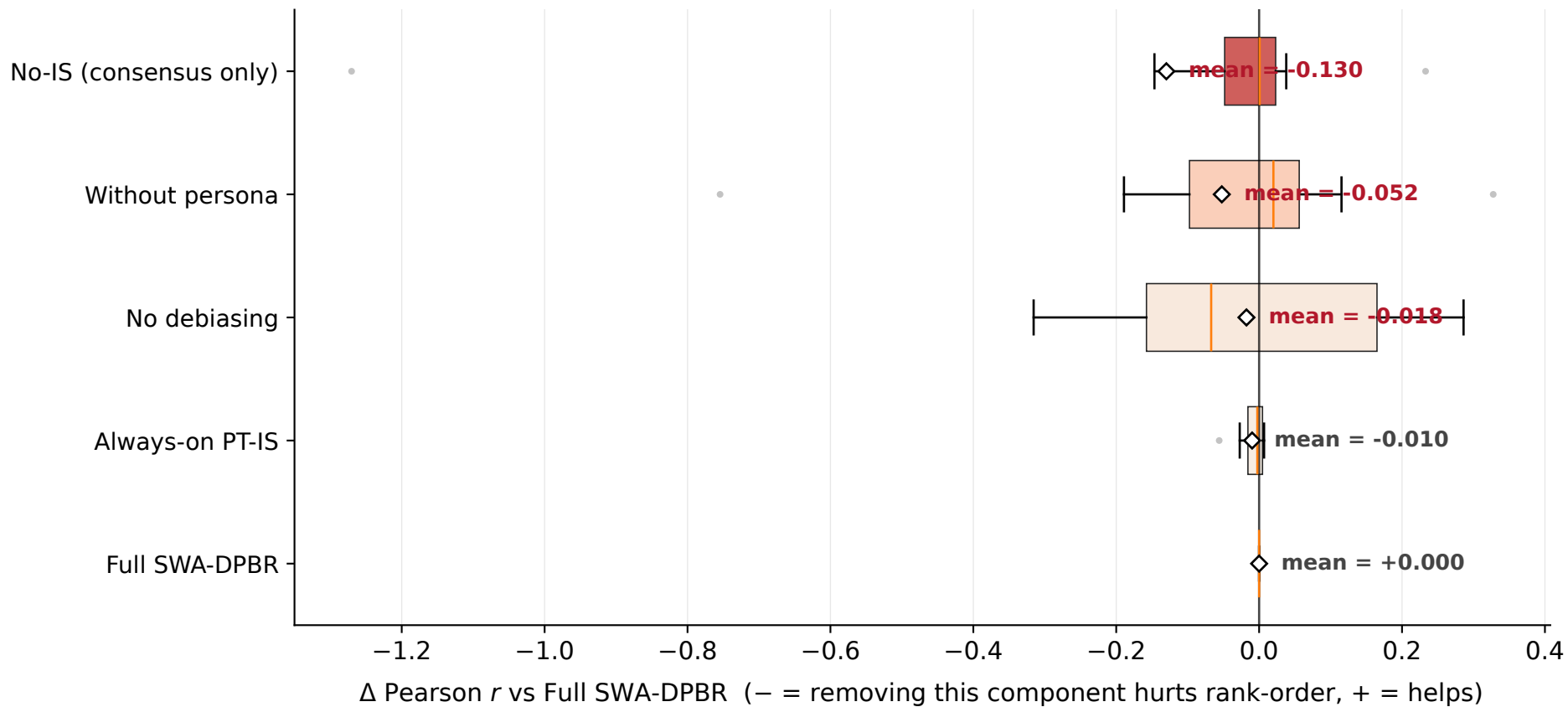
Ablation effect on rank-order alignment ( \Delta Pearson r , 3 models \times 3 countries)
