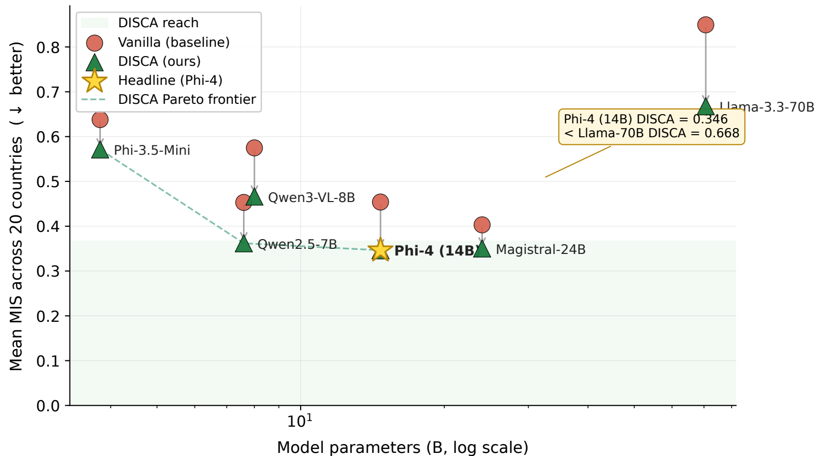
Calibration competes with scale — DISCA reshapes the size/MIS curve
