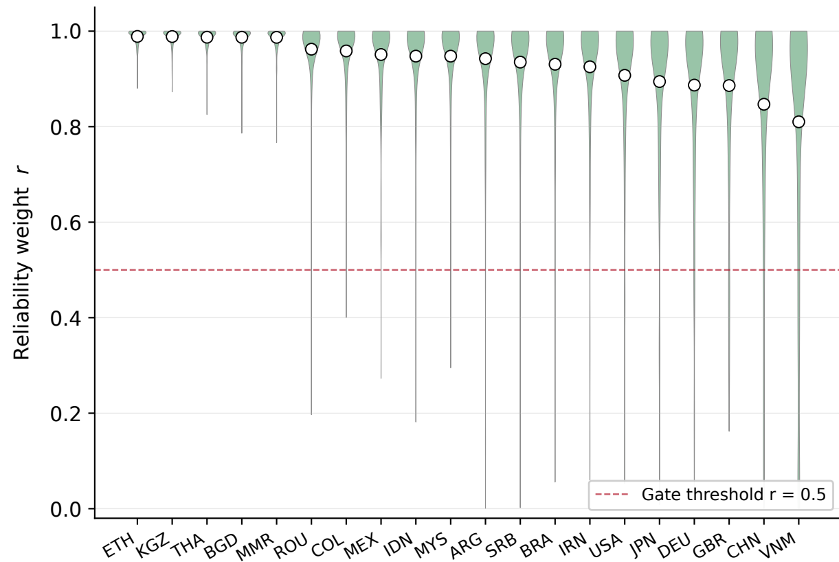
Per-country distribution of r (Phi-4 (14B))
