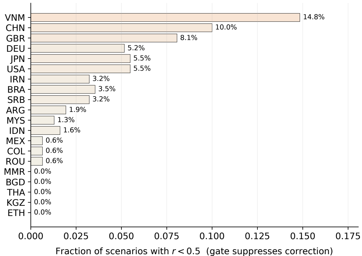
DPBR self-regulation: where the gate intervenes
