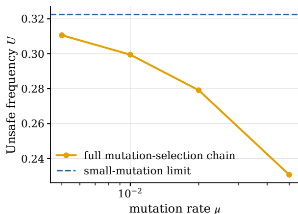
C the small-mutation reduction
