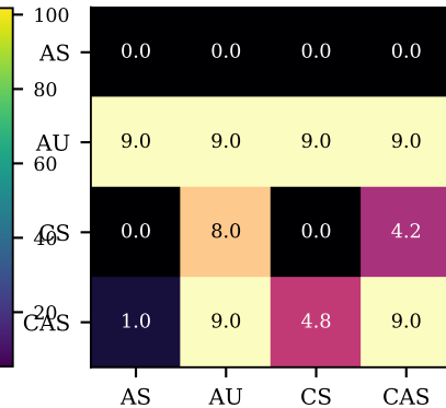
unsafe actions m(i,j)
