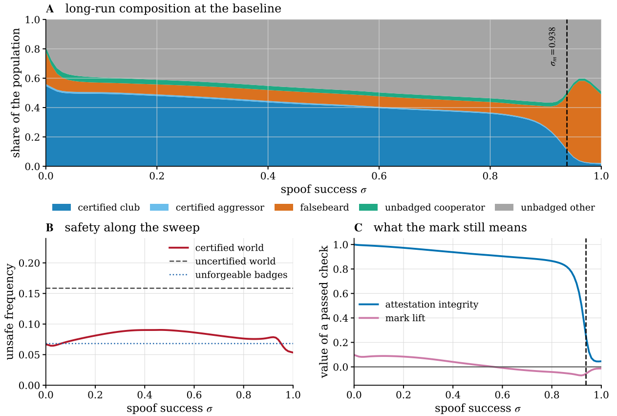
Figure 5: The certification cliff. (A) Long-run composition against spooft success; the dashed line is the mimicry threshold \sigma_m = 0.938 . (B) Unsafe frequency of the certified world against the uncertified world and against a counterfactual in which badges cannot be forged. (C) The two things a passed check can be worth. Attestation integrity, the posterior that a passed badge is genuine, survives until \sigma_m ; the mark lift, the behavioural value of a passed check, is already negative at \sigma = 0.57 .
