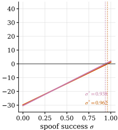
B clustered ( r=0.1 )
