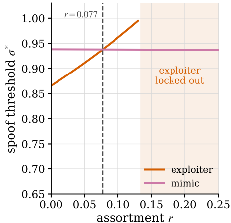
C clustering flips it
