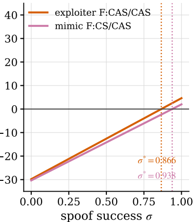
A well mixed ( r=0 )
