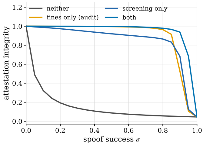
B the channels along the sweep ( \rho=20 )
