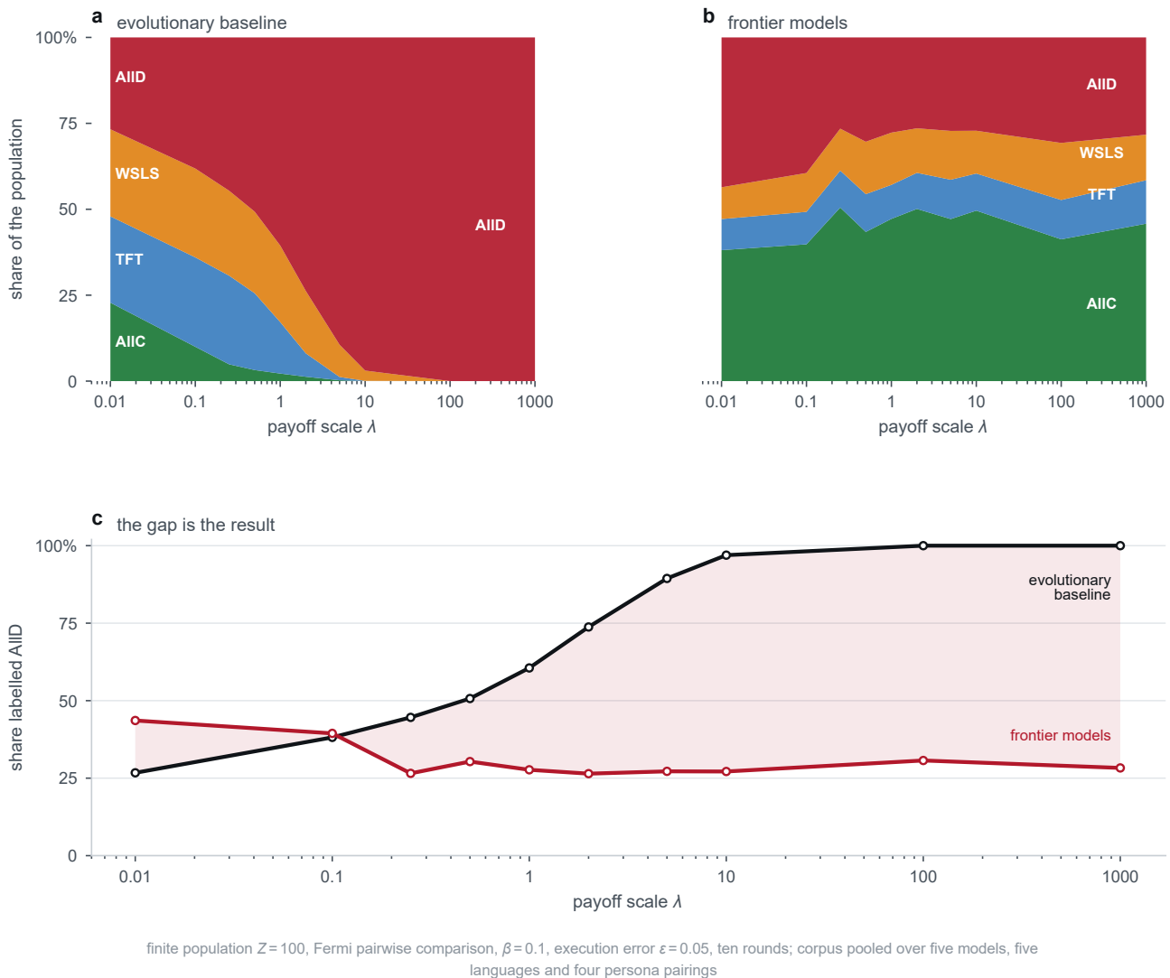
Figure 6. The evolutionary baseline and the corpus move in opposite directions. (a) The baseline's stationary distribution over the four canonical rules across the ten payoff scales, drawn as a stacked band. (b) The corpus's strategy mix on the same axis, drawn identically. (c) The AIID share alone, both accounts on one axis, with the gap shaded. Baseline at Z = 100 , \beta = 0.1 , \epsilon = 0.05 , ten rounds; the corpus pooled over five models, five languages and four persona pairings.
