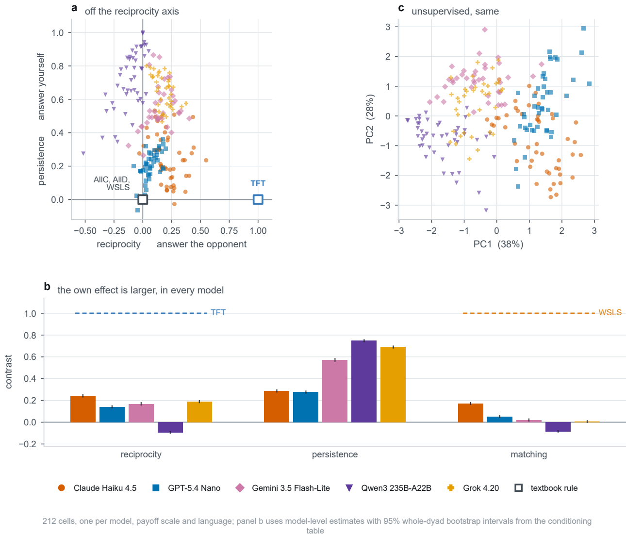
Figure 7. Own-action conditioning exceeds partner-action conditioning at the model level. (a) Cells in the reciprocity by persistence plane, with the canonical rules at their exact coordinates; AIIC, AIID and win-stay lose-shift all have both main effects zero and so coincide at the origin. (b) The three contrasts per model, against the value each canonical rule would give, with 95% percentile intervals from whole-dyad bootstrap resampling. (c) The first two principal components of the raw five-vector, which is given no knowledge of the contrasts and recovers the same geometry. Panels (a) and (c) use model-by-scale-by-language cells; a predecessor observed fewer than thirty times yields no estimate and the cell is dropped, leaving 212 of 250.
