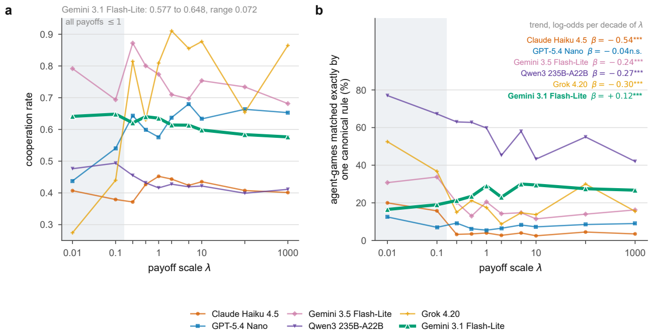
Figure B.1. The sixth model beside the five reported in the main text. Gemini 3.1 Flash-Lite is drawn heavier and in front. (a) Cooperation against the payoff scale, where it sits inside the spread of the other five. (b) Share of agent-games matched exactly by one canonical rule, with each model's trend per decade of \lambda . It is the only model of the six whose trend is positive.
