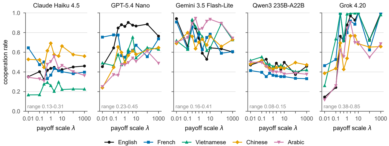
Figure 3. Cooperation against the payoff scale, by model and prompt language. One panel per model, one curve per prompt language; the annotation gives the smallest and largest across-scale range among that model's five languages. Each point averages 40 dyads.
