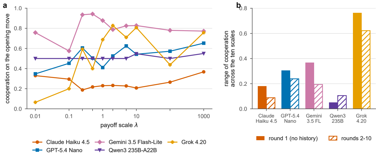
Figure 8. Cooperation on the opening move, against the payoff scale. At round 1 the agent has seen only the matrix and the instructions. (a) Cooperation on the opening move, one curve per model. (b) Range of cooperation across the ten scales, on the opening move (solid) and over rounds 2 to 10 (hatched).
