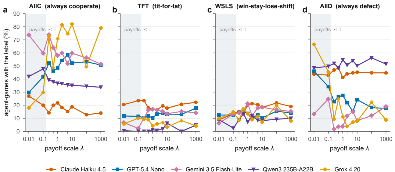
Figure 7. Share of agent-games carrying each canonical label, against the payoff scale. One panel per canonical rule: (a) AIIC, (b) Tit-for-Tat, (c) Win-Stay-Lose-Shift, (d) AIID. Each point is the share of that model's 400 agent-games at that scale carrying the label, and shaded bands mark the two scales at which every payoff printed is at most 1. The AIIC and AIID panels rest partly on exact rule matching, whereas over the corpus 94.6% of the Tit-for-Tat labels and 97.1% of the Win-Stay-Lose-Shift labels are attributions made where no canonical rule fits, so those two panels should be read as a resemblance rather than as an identification.
