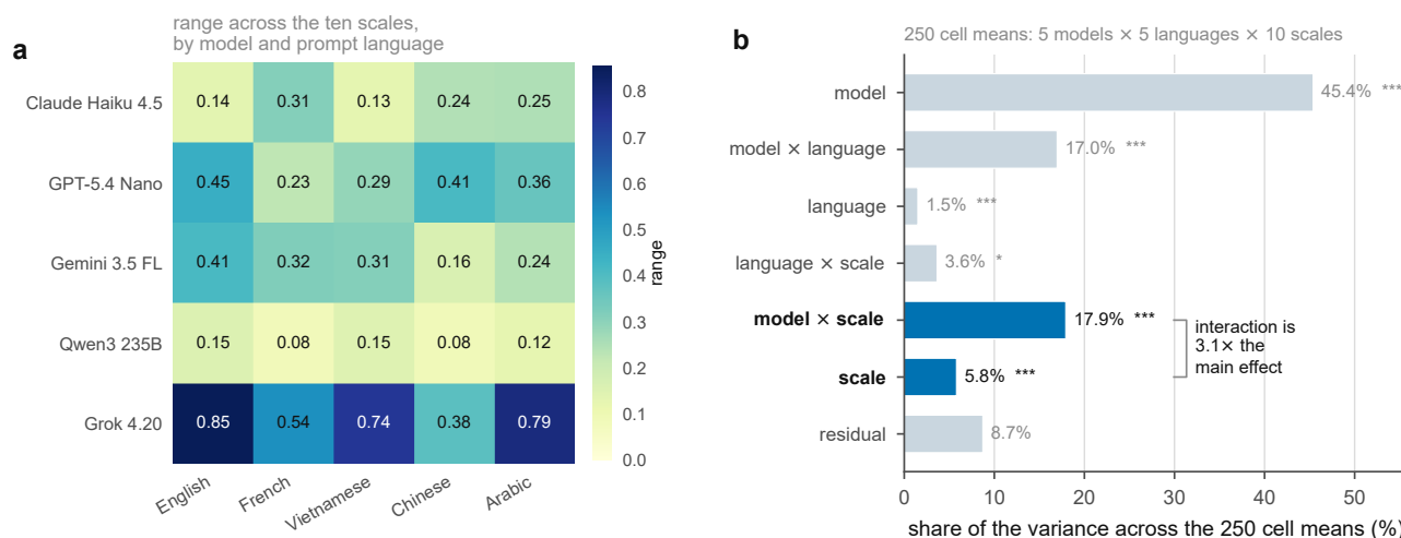
Figure 4. Where the movement lives. (a) Across-scale range of cooperation for each model-by-language pair; the range of the ranges is an order of magnitude, from 0.083 to 0.855. (b) Share of the variance across the 250 cell means carried by each term of a type-II analysis of variance. The interaction of the payoff scale with the model carries about three times what the scale main effect carries.
