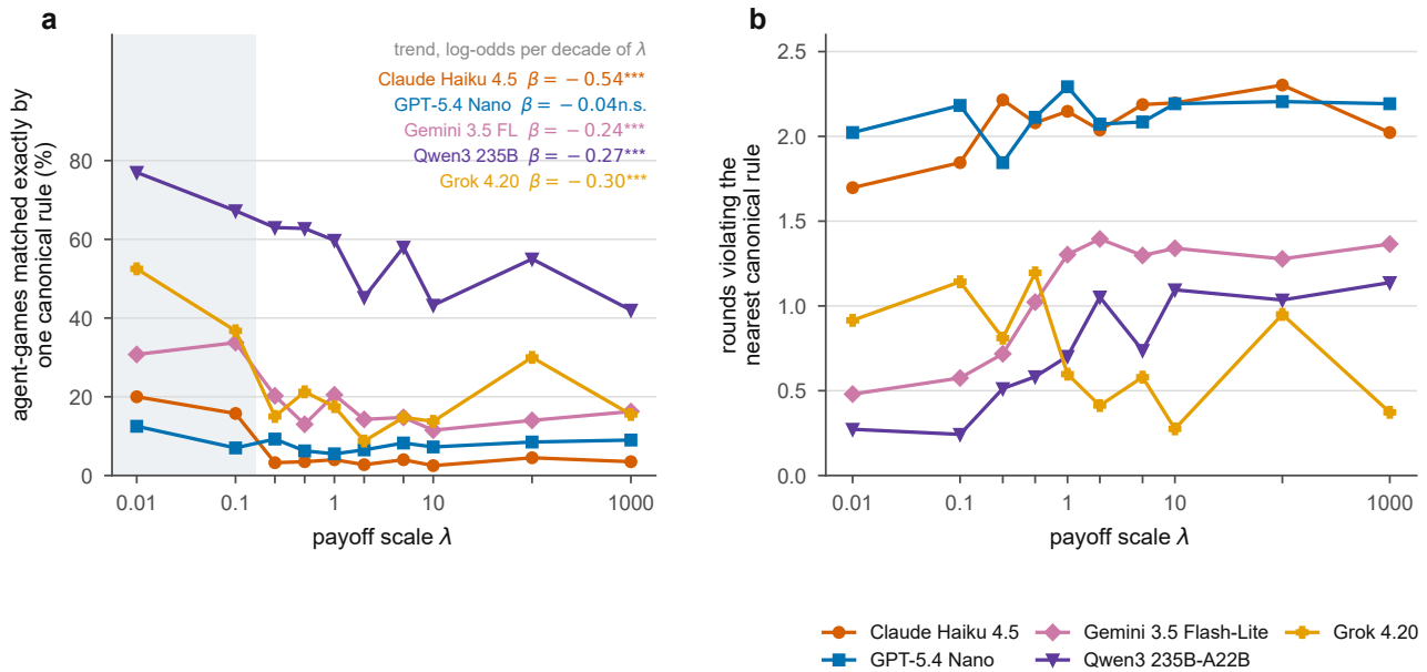
Figure 6. How closely play follows the canonical memory-one rules, against the payoff scale. Both panels are computed by exact matching, with no learned component. (a) Share of agent-games matched exactly by one canonical rule, one line per model, annotated with that model's trend per decade of \lambda ; all five trends are negative, and only in GPT-5.4 Nano is the trend not distinguishable from zero (table 3). The shaded band marks the two scales at which every payoff printed is at most 1. (b) Mean number of rounds, out of the ten played, violating the nearest canonical rule. Here the trends do not all have the same sign: Grok 4.20 runs against the other four (table 3).
