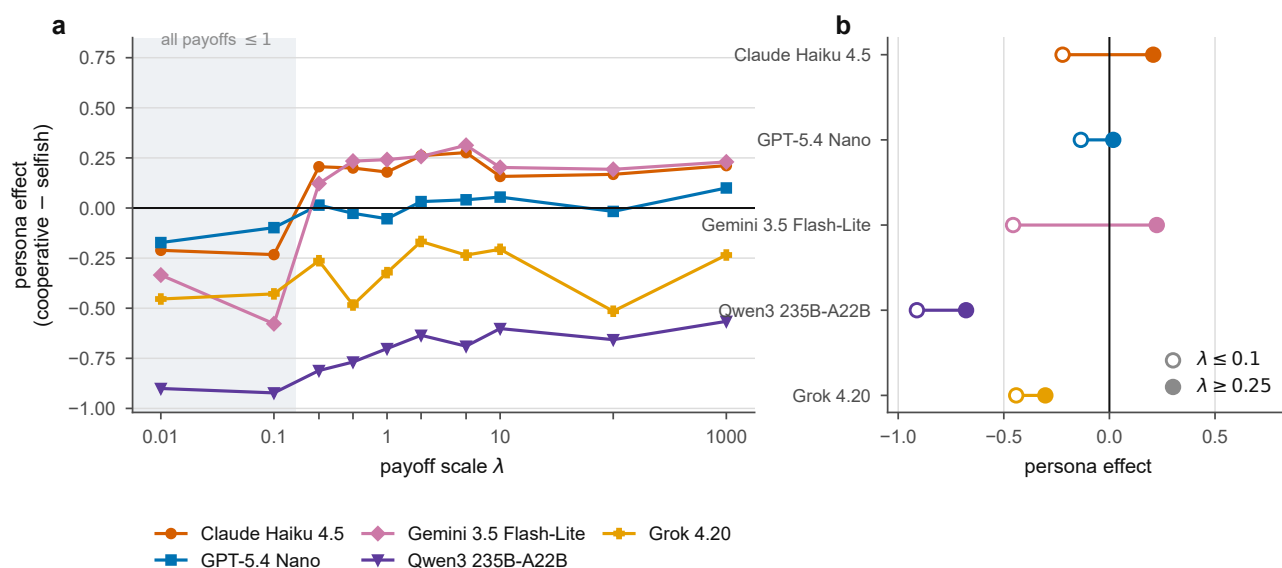
Figure 5. The persona effect against the payoff scale. The persona effect is the cooperation rate under a cooperative persona minus that under a selfish one. (a) The effect against the payoff scale, each point averaging 200 dyads; the shaded band marks the two scales at which every payoff printed is at most 1. (b) The same contrast as two regime means: open markers at \lambda \leq 0.1 , filled markers at \lambda \geq 0.25 (table 2).
