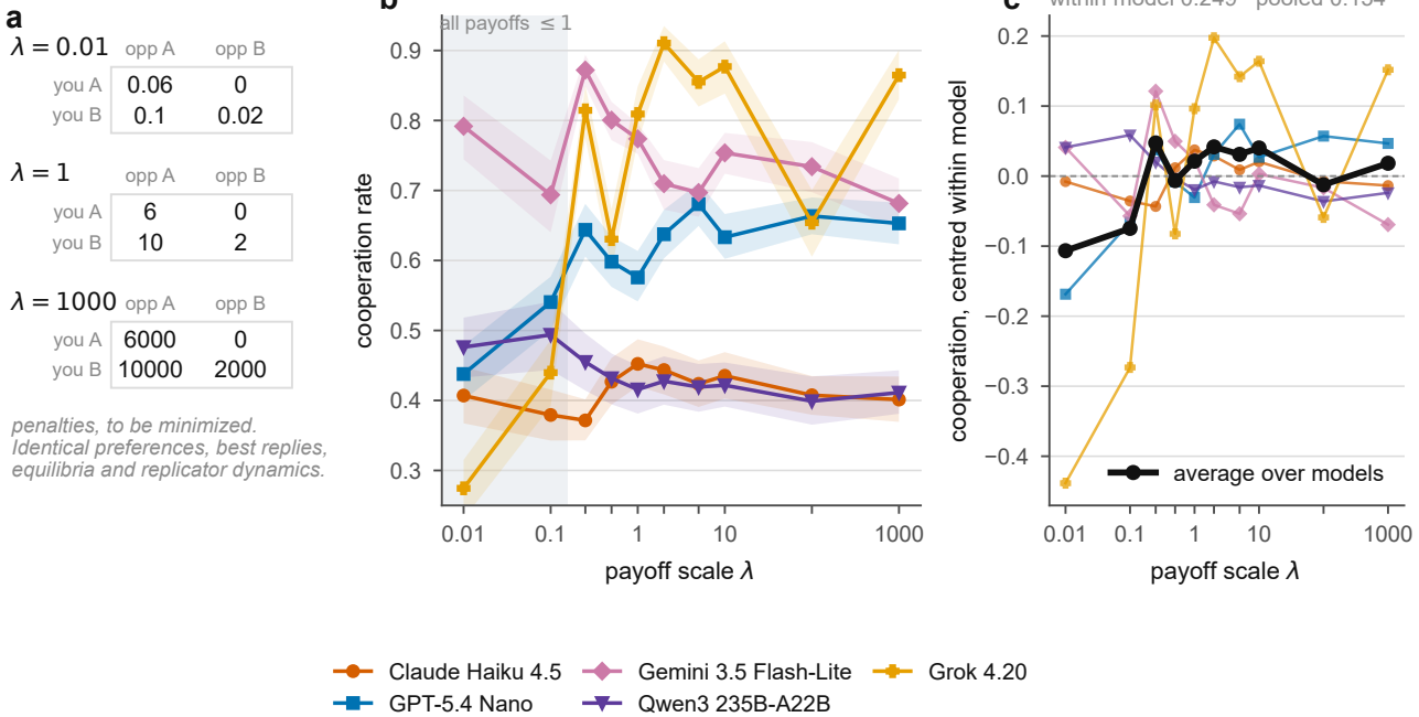
Figure 1. Cooperation against the payoff scale in five language models. (a) The same prisoner's dilemma at three payoff scales, shown to the agent as penalties to be minimised. (b) Cooperation against the payoff scale, one curve per model; the shaded band marks the two scales at which every payoff printed is at most 1. (c) The curves of (b) centred within model, with their average in black. Each point in (b) and (c) averages 200 dyads; the envelope around each curve in (b) is a 95% percentile interval from 1,500 bootstrap resamples of whole dyads.
