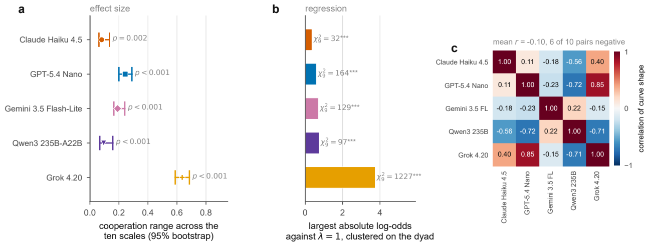
Figure 2. The departure from invariance, tested three ways. (a) Across-scale range of cooperation per model, with a 95% interval from the dyad bootstrap and the p value of a permutation test that shuffles the payoff scale among whole dyads; 0.0005 is the smallest value 2,000 draws can return. (b) Largest absolute log-odds contrast against \lambda = 1 in a per-model logistic regression of the round-level decision, with the clustered Wald statistic on its nine scale contrasts. (c) Correlation between the ten-point curve shapes of each pair of models, after centring each curve within model. Six of the ten pairs are negative.
