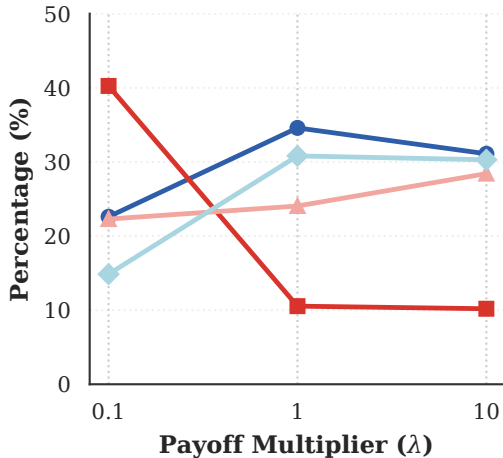
Claude 3.5
