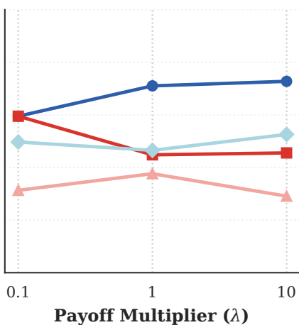
Mistral
