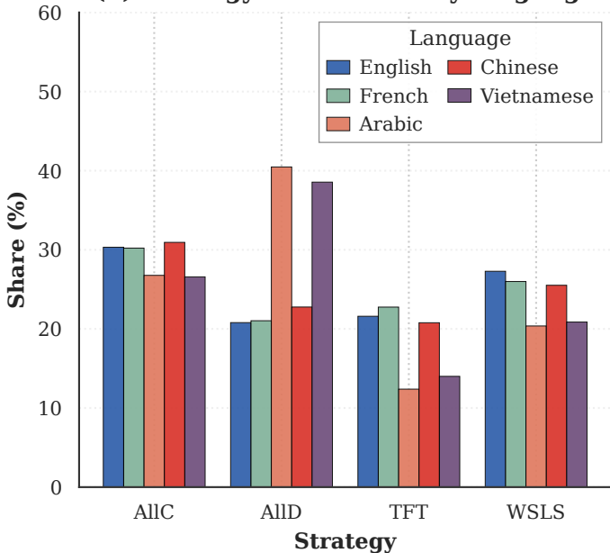
(b) Strategy distribution by language
