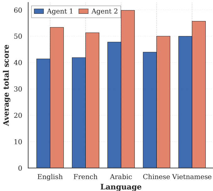
(a) Average score by language
