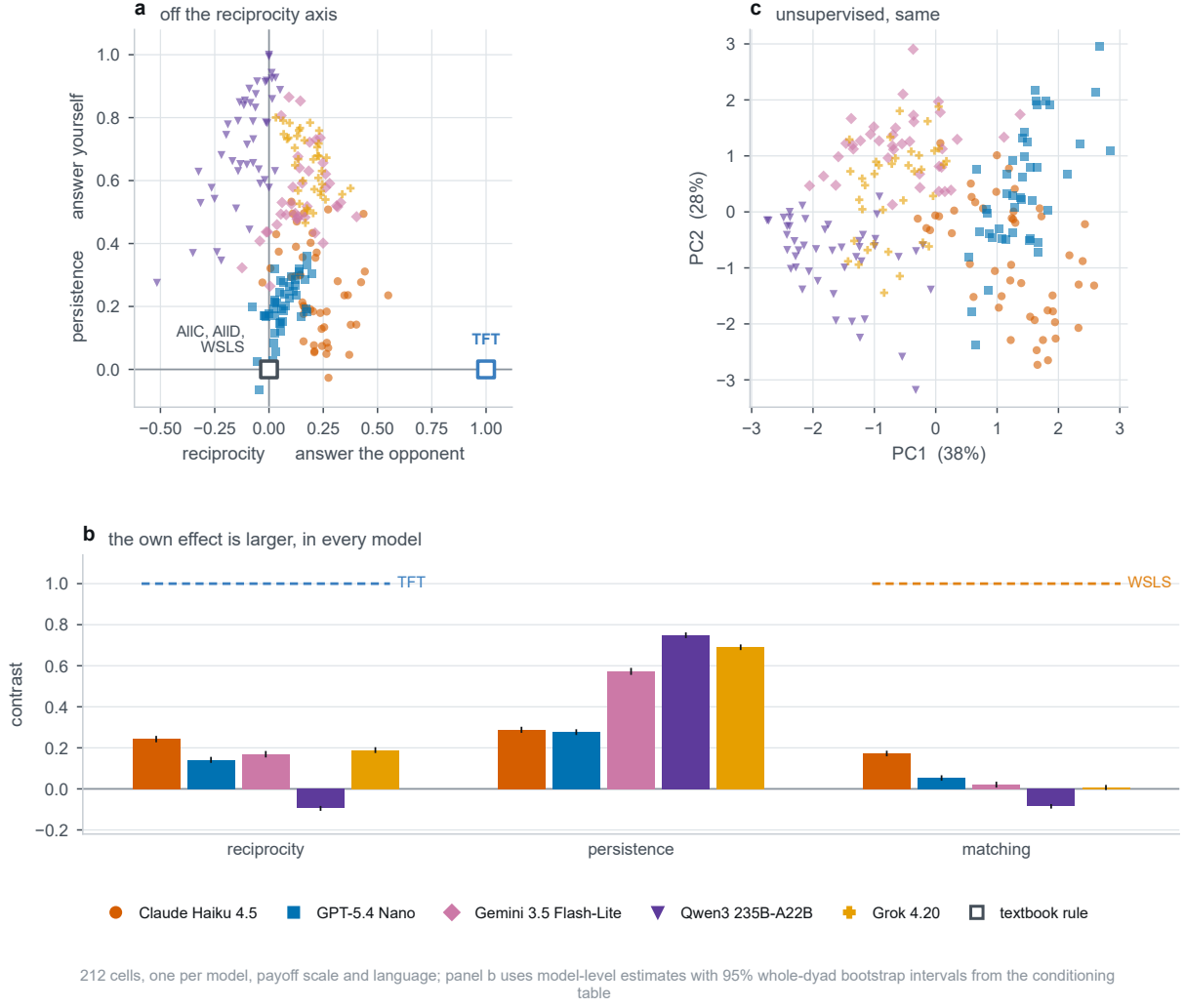
Figure 7: Own-action conditioning exceeds partner-action conditioning at the model level. (a) Cells in the reciprocity by persistence plane, with the canonical rules at their exact coordinates; AllC, AllD and win-stay lose-shift all have both main effects zero and so coincide at the origin. (b) The three contrasts per model, against the value each canonical rule would give, with 95% percentile intervals from whole-dyad bootstrap resampling. (c) The first two principal components of the raw five-vector, which is given no knowledge of the contrasts and recovers the same geometry. Panels (a) and (c) use model-by-scale-by-language cells; a predecessor observed fewer than thirty times yields no estimate and the cell is dropped, leaving 212 of 250.
