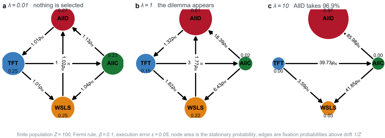
Figure 10. Where the payoff scale does act: the invasion structure of a finite population. Nodes are the four monomorphic states, node area is the small-mutation-limit stationary probability, and an edge is drawn where a single mutant fixes more often than neutral drift 1/Z would carry it, labelled in multiples of that drift. Z = 100 , Fermi pairwise comparison, \beta = 0.1 , \epsilon = 0.05 . Because \lambda and \beta enter the update rule only through their product, raising the scale is raising selection pressure. The panels stop at \lambda = 10 because the float64 fixation probabilities underflow beyond it; those cells are solved at 200 digits instead (appendix C).
