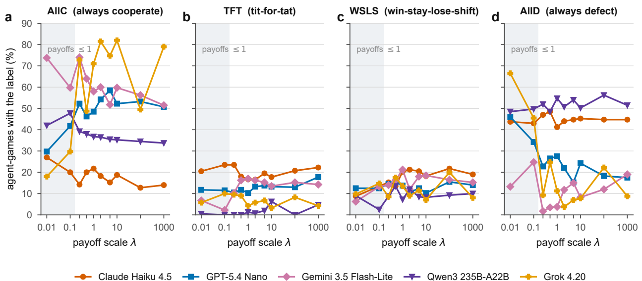
Figure 7. Share of agent-games carrying each canonical label, against the payoff scale. One panel per canonical rule: (a) AIIC, (b) Tit-for-Tat, (c) Win-Stay-Lose-Shift, (d) AIID. Each point is the share of that model's 400 agent-games at that scale carrying the label, and shaded bands mark the two scales at which every payoff printed is at most 1. The AIIC and AIID panels rest partly on exact rule matching, whereas over the corpus 94.6% of the Tit-for-Tat labels and 97.1% of the Win-Stay-Lose-Shift labels are attributions made where no canonical rule fits, so those two panels should be read as a resemblance rather than as an identification.
