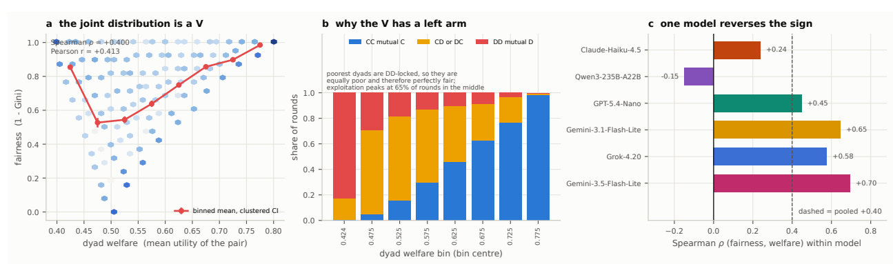
Figure B.4. Outcome fairness, net exploitation and the V-shaped welfare frontier. (a) Within-dyad fairness ( 1 - \text{Gini} ) plotted against joint dyad welfare across all experimental conditions, revealing a characteristic V-shaped relationship where equality peaks at both mutual defection (low welfare) and mutual cooperation (high welfare), with inequality concentrated in the exploitative transition zone. (b) Per-model fairness trajectories showing how different models occupy distinct regimes along the welfare-fairness frontier. (c) Distributional equity across the ten payoff scales: the fitted association is small and imprecise (slope 0.0004, p = 0.80 ).
