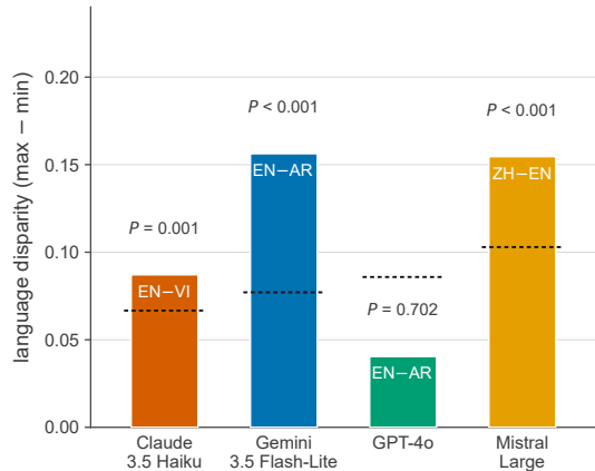
Language disparity against chance ---- 95th pct. of permutation null
