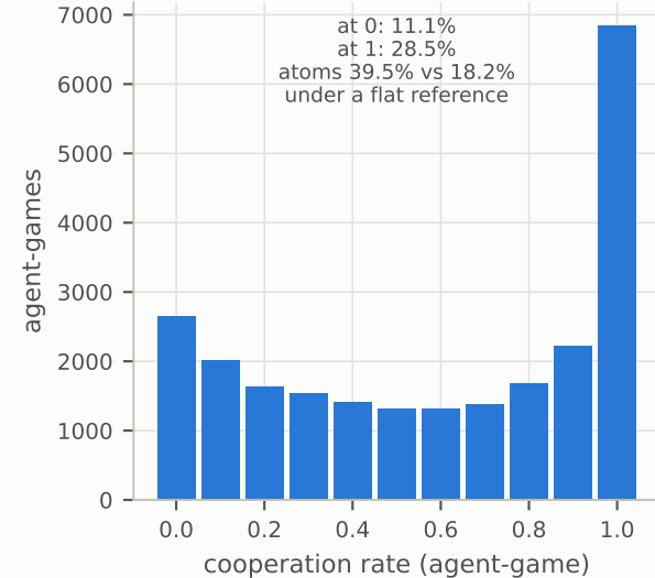
a pooled: U-shaped and top-heavy
