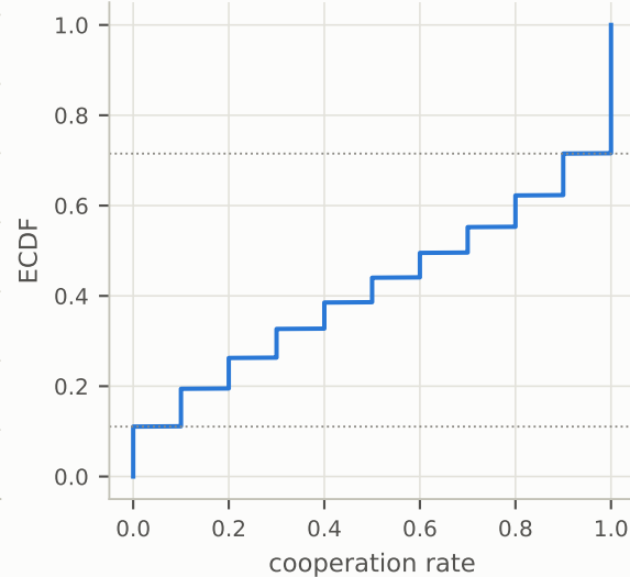
b ECDF: two vertical jumps
