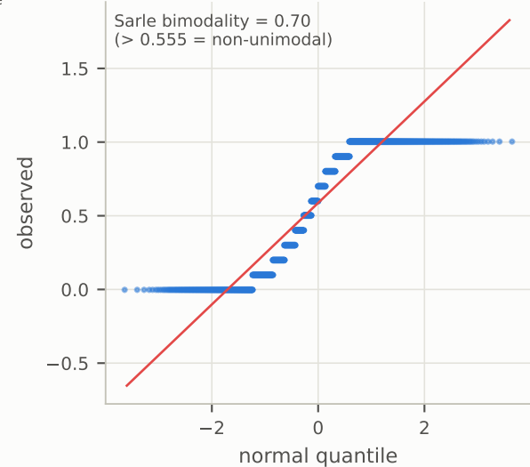
d Q-Q: far from Gaussian
