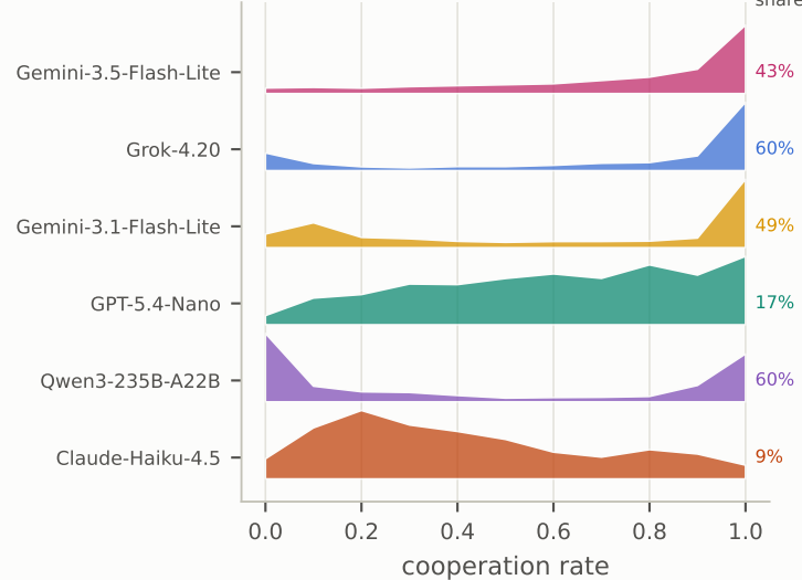
c the shape is model-specific
