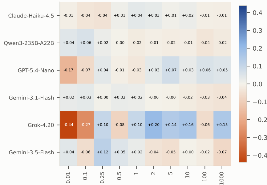
a model \times \lambda
