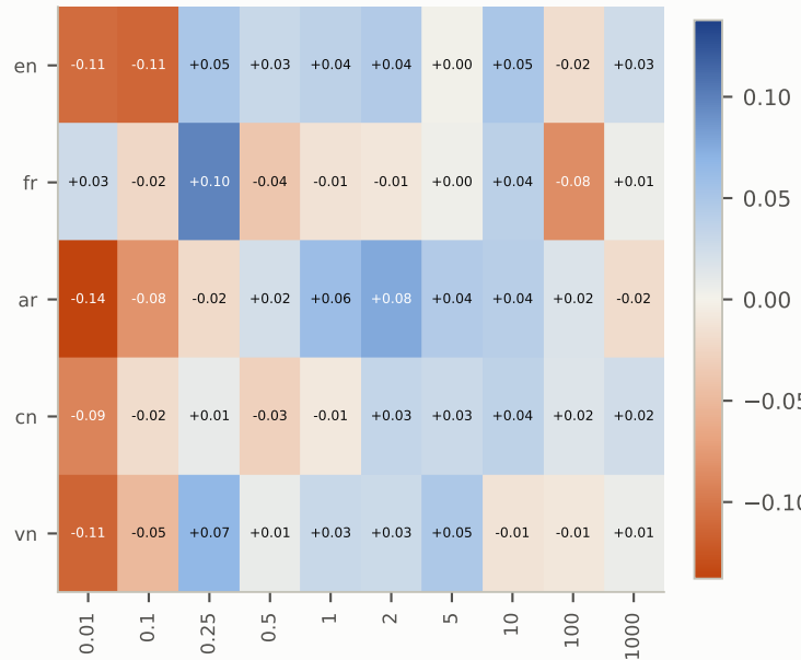
b language \times \lambda
