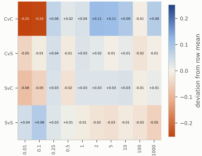
c pairing \times \lambda
