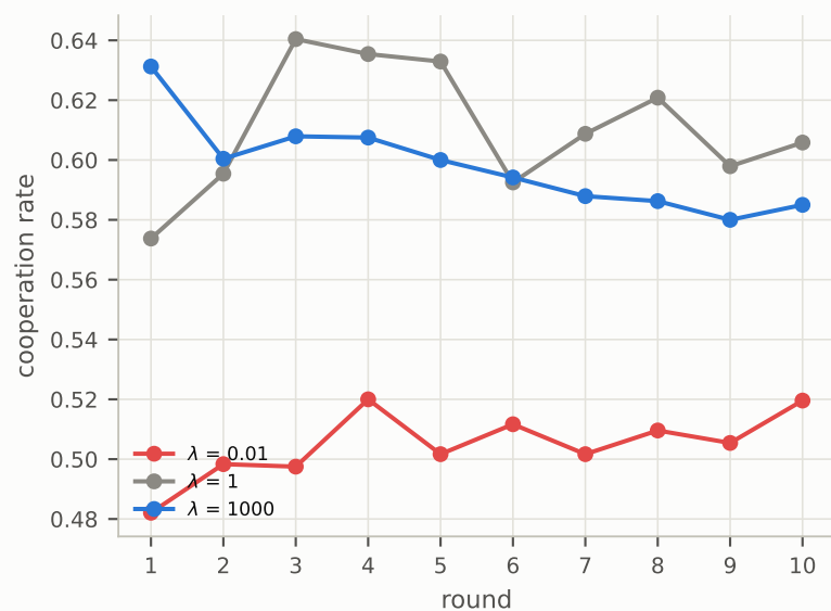
c \lambda shifts the level, not the decay
