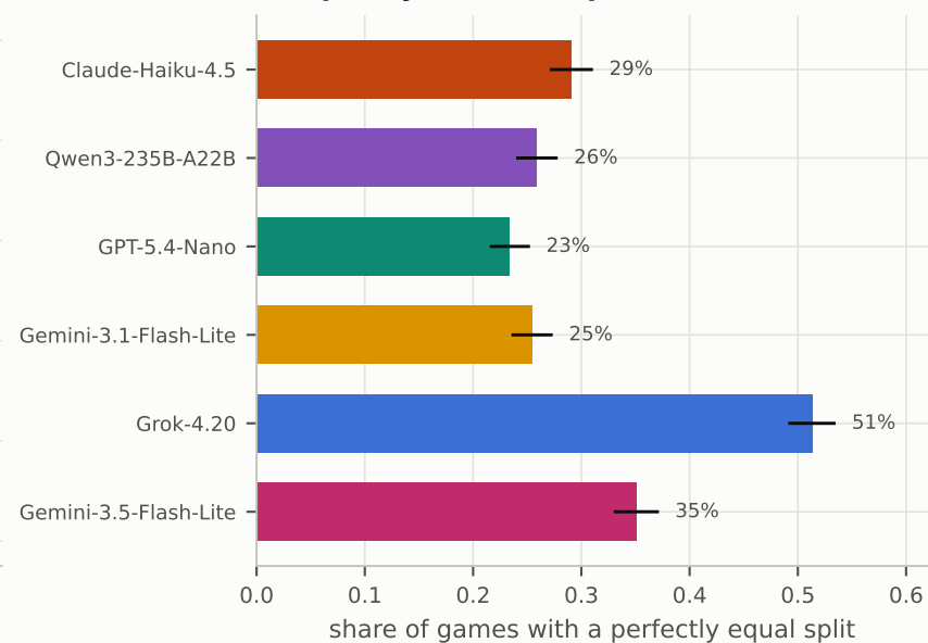
c equality is model-specific
