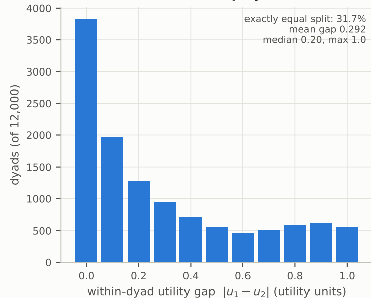
a outcome fairness is spiky
