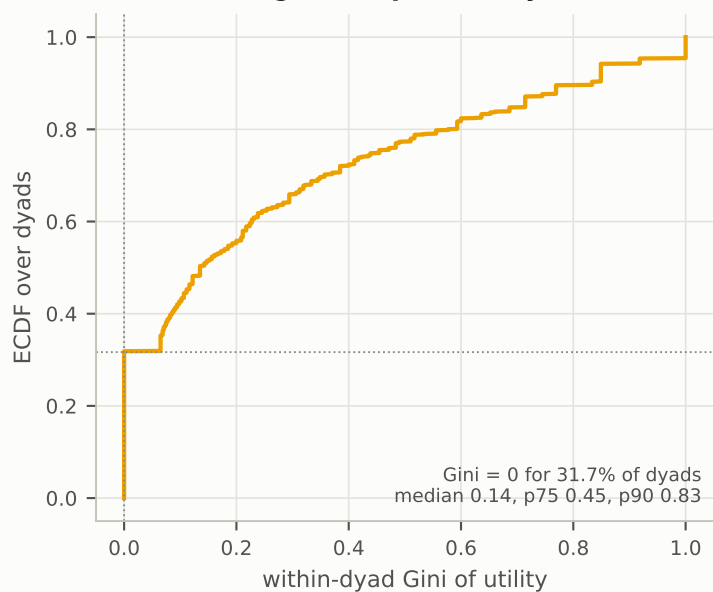
b a third of games split evenly
