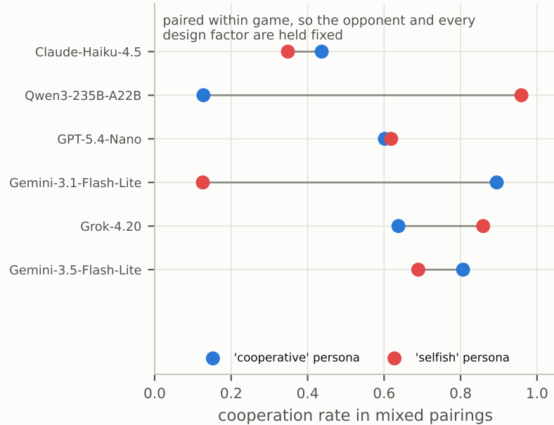
a what the persona label does
