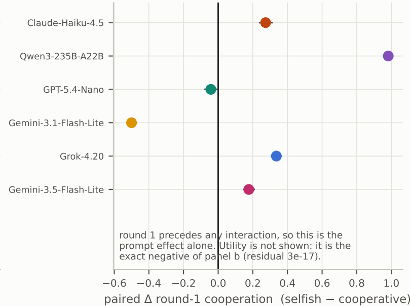
c the label acts on the opening move
