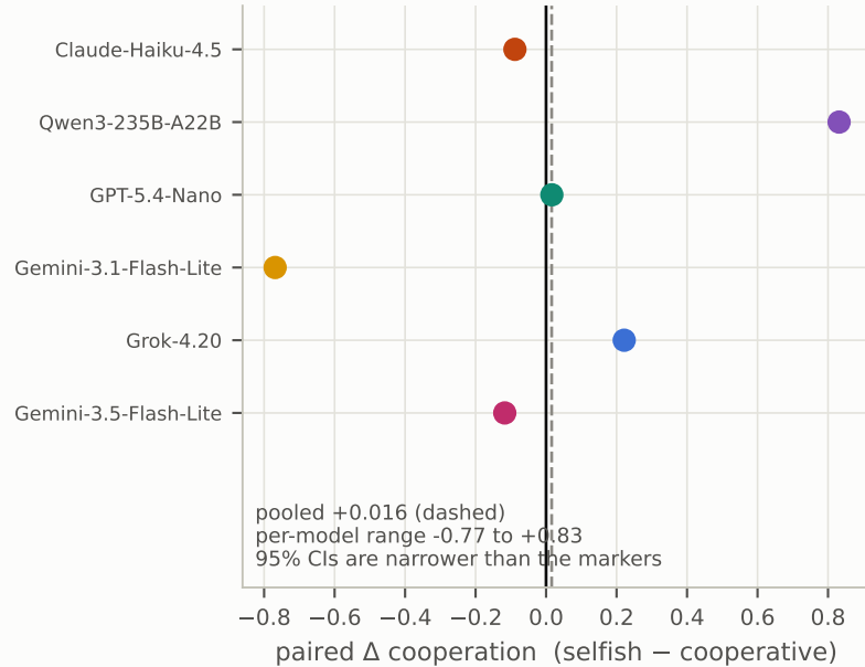
b the pooled effect is an artefact
