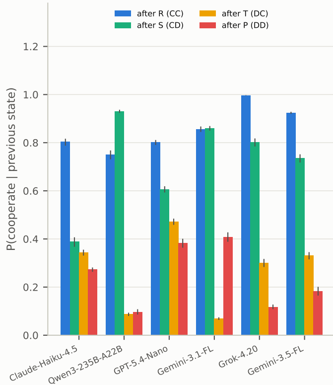
b with game-clustered 95% CIs
