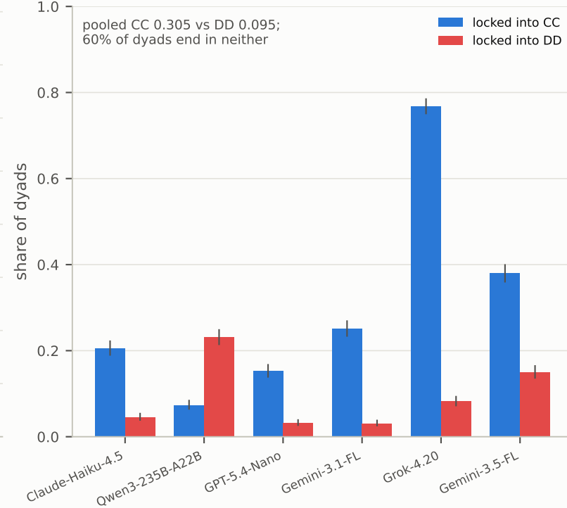
b cooperation locks in more often
