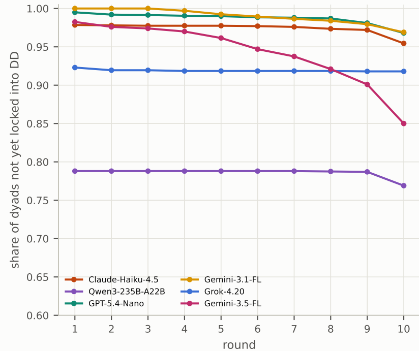
a survival against DD lock-in
