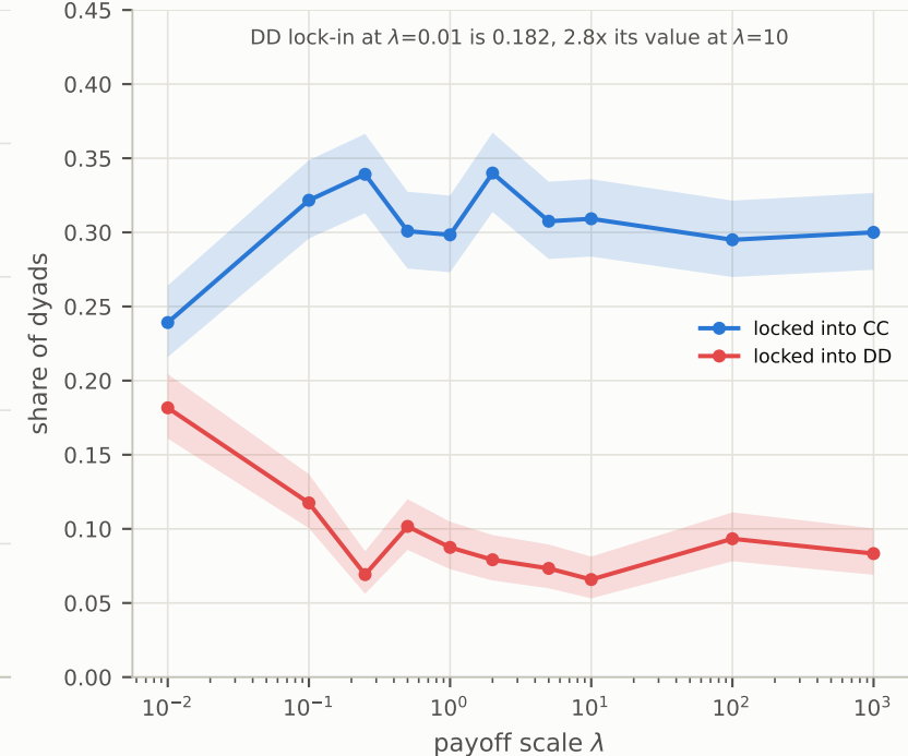
c lock-in across \lambda
