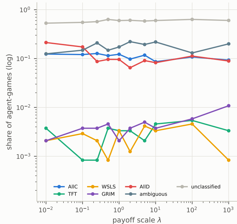
a strategy shares across \lambda
