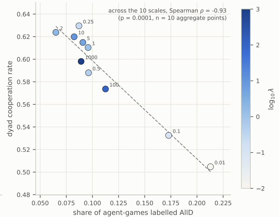
c the \lambda effect runs through AIID
