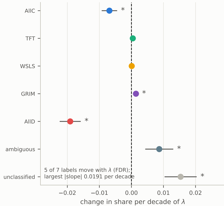
b slopes with 95% CI
