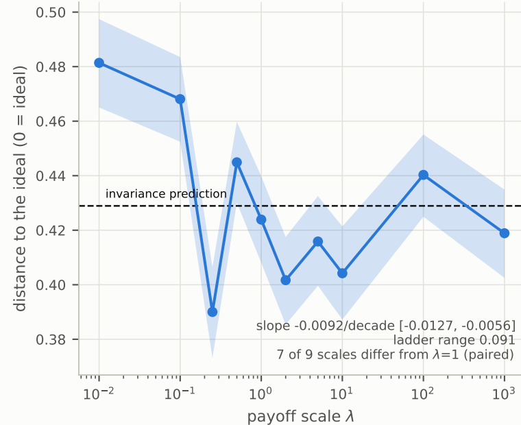
a distance vs \lambda
