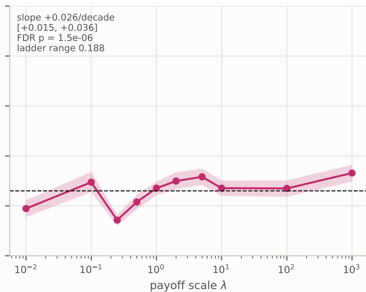
Gemini-3.5-Flash-Lite
