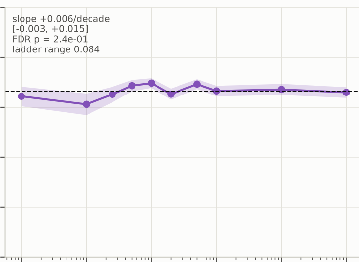
Grok-4.20-Non-Reasoning
