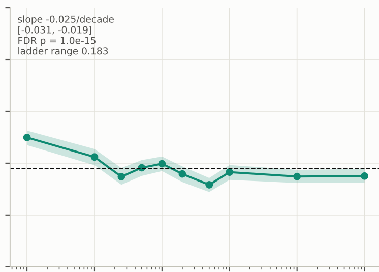
Gemini-3.5-Flash-Lite
