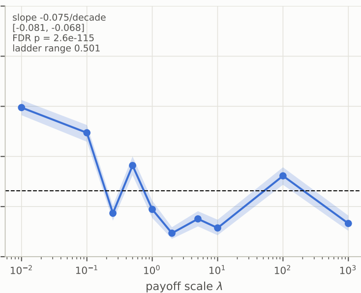
Grok-4.20-Non-Reasoning
