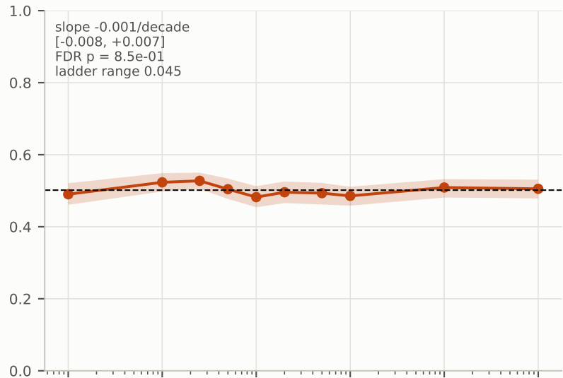
Gemini-3.1-Flash-Lite
