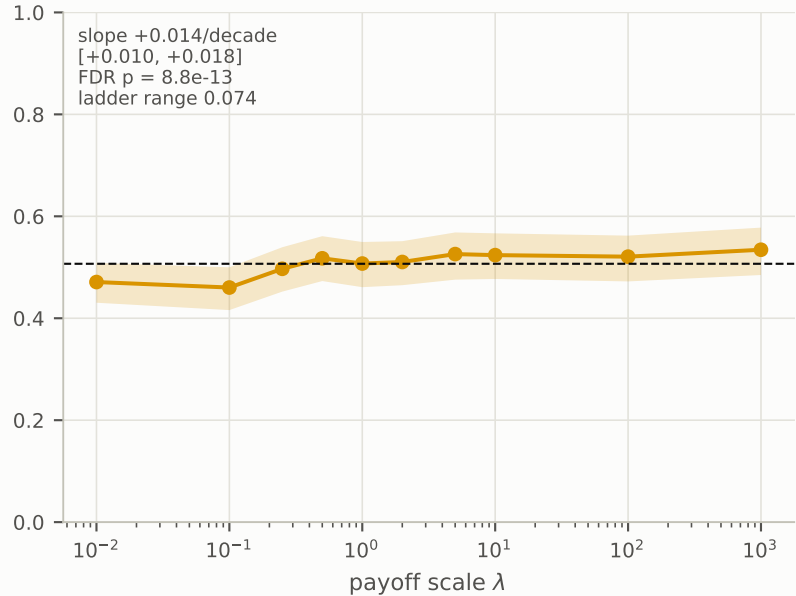
Gemini-3.1-Flash-Lite
