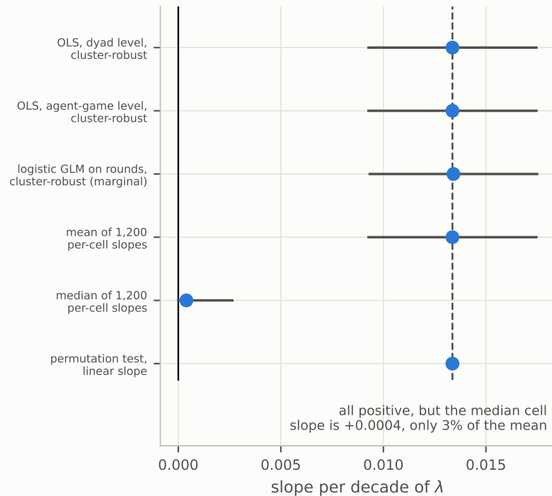
a six estimators, same units
