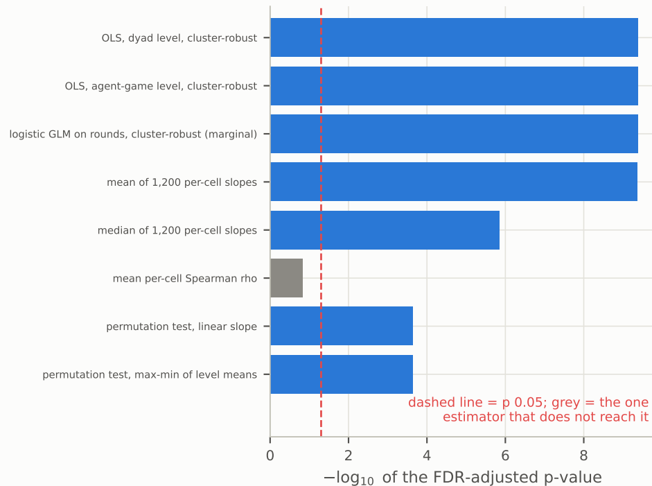
b 7 of 8 survive FDR adjustment
