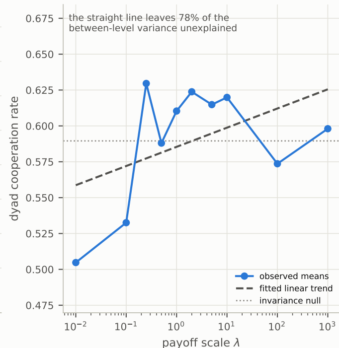
c why the linear fit is a poor summary
