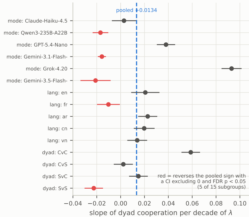
a the pooled \lambda slope reverses
