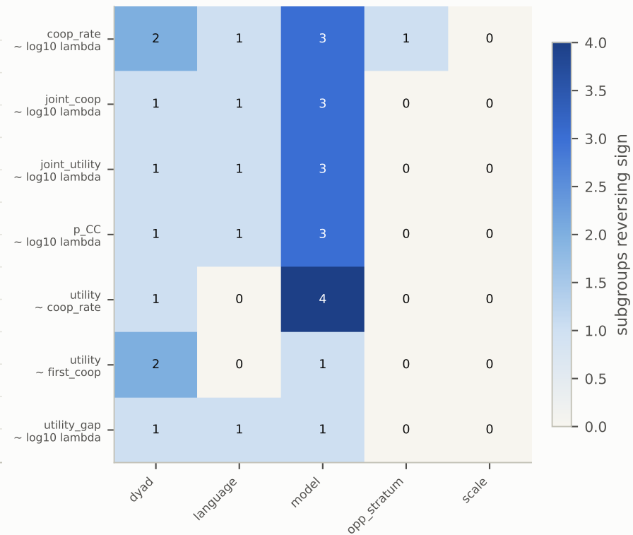
c reversals found, by search cell
