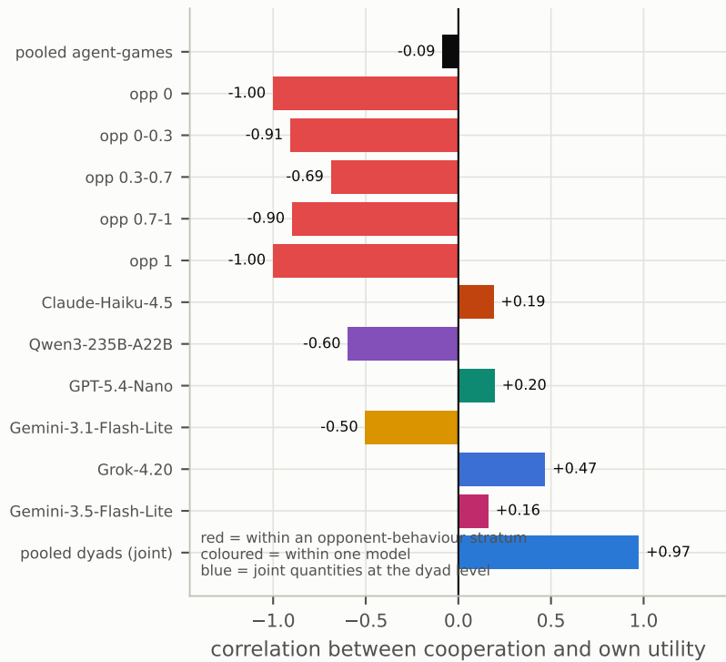
b same variable pair, opposite signs
