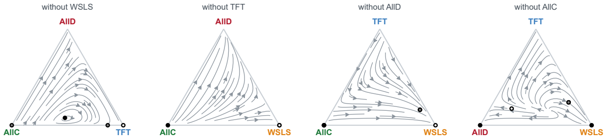
Figure C.1. The deterministic dynamics do not see the payoff scale. Replicator flow on each of the four faces of the three-simplex spanned by the canonical rules, one face per strategy left out, at \lambda = 1 , \varepsilon = 0.05 and ten rounds. Filled circles are stable rest points, open circles unstable. Only one row is drawn because rescaling the payoffs multiplies the field by a constant and moves nothing: the matrix at \lambda = 1000 is exactly 10^5 times the matrix at \lambda = 0.01 , and over 2,000 random population states the normalised fields agree to 4 \times 10^{-14} .
