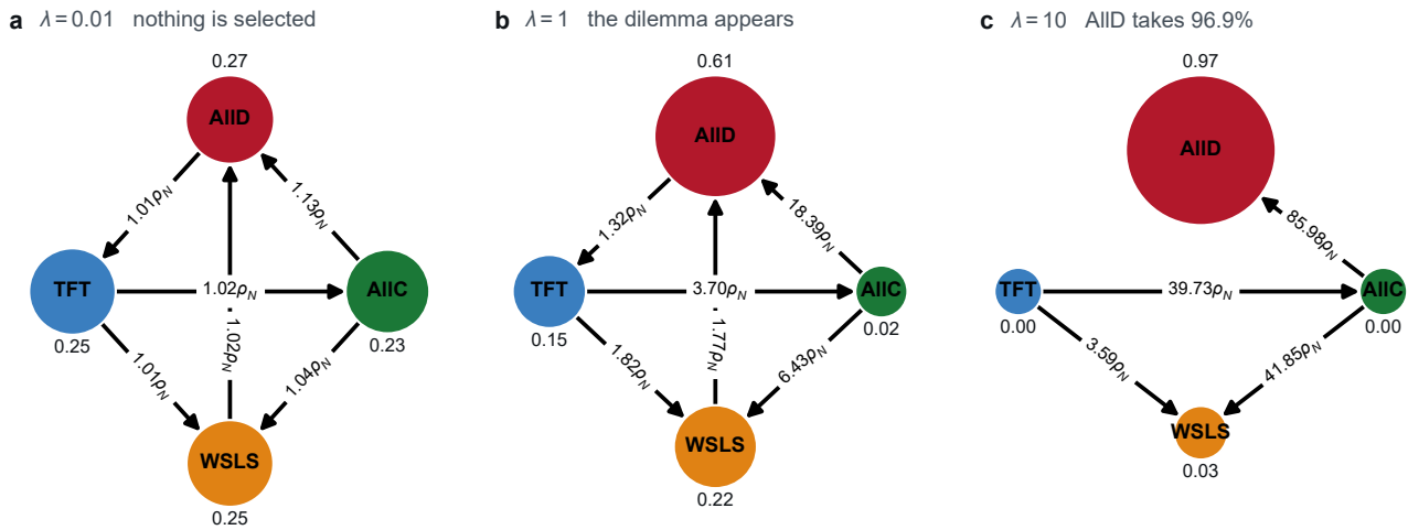
Figure C.2. Where the payoff scale does act: the invasion structure of a finite population. Nodes are the four monomorphic states, node area is the small-mutation-limit stationary probability, and an edge is drawn where a single mutant fixes more often than neutral drift 1/Z would carry it, labelled in multiples of that drift. Z = 100 , Fermi pairwise comparison, \beta = 0.1 , \varepsilon = 0.05 . Because \lambda and \beta enter the update rule only through their product, raising the scale is raising selection pressure. The panels stop at \lambda = 10 because the float64 fixation probabilities underflow beyond it; those cells are solved at 200 digits instead.
