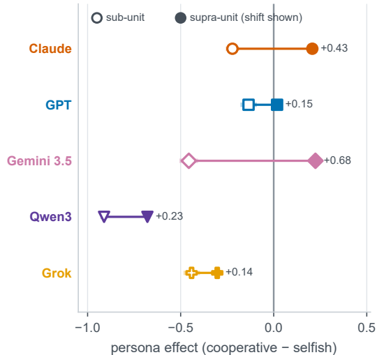
b regime shift: sub-unit vs supra-unit
